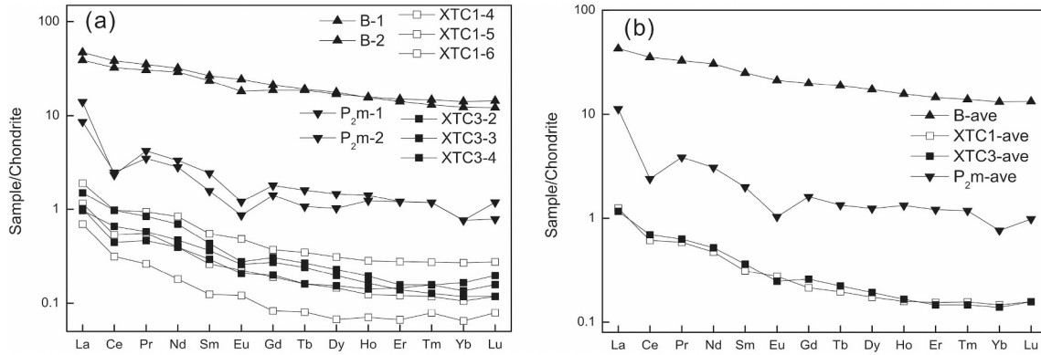
Fig. 6. Chondrite-normalized REE profiles for basalts (B-1 and B-2), chalcopyrites (XTC1 from No. 1 ore body, XTC3 from No. 3 ore body) and limestone ( \text{P}_2\text{m} ) from the Maokou formation (Xiao, 2005). (a) Pattern for each individual sample; (b) pattern for average REEs of each type samples.
