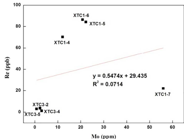
Fig. 7. Re vs. Mo diagram for chalcopyrite samples from the No. 1 and 3 ore bodies in the Xiaotongchang deposit.
