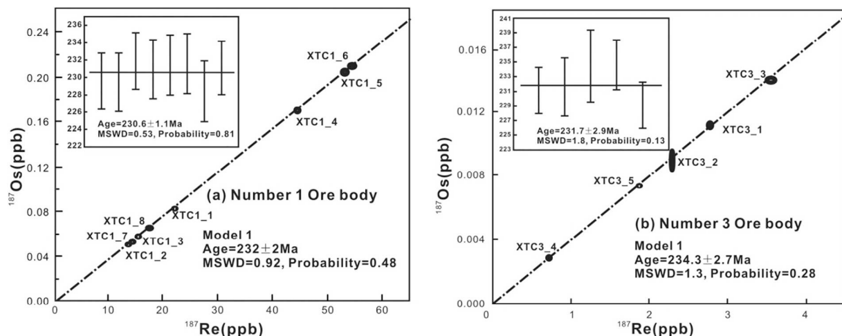
Fig. 5. ^{187}\text{Re} - ^{187}\text{Os} (parent-daughter) isochron diagrams and weighted average model age diagrams for chalcopyrite samples. (a) No. 1 ore body in Xiaotongchang deposit. (b) No. 3 ore body in Xiaotongchang deposit.
