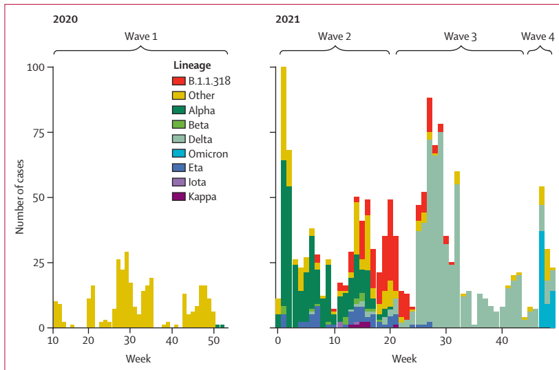
Figure 2: SARS-CoV-2 lineage distribution across four COVID-19 waves in Ghana Number of cases caused by each lineage during each week of 2020 (starting at week 10) and each week of 2021. Data are from a subset of 692 samples sequenced in the current study, and 1123 samples collected in Ghana by Morang'a and colleagues. 35 Wave 1 (April to December, 2020) was driven by early variants (eg, B.1 and B.1.1 were most dominant), whereas wave 2 (January to April, 2021), wave 3 (May to November, 2021), and wave 4 (November to December, 2021) were driven by variants of concern and variants of interest; alpha (B.1.1.7), beta (1.351), delta (B.1.617.2), and omicron (B.1.1.529) were designated as variants of concern, and eta (B.1.525), iota (B.1.526), and kappa (B.1.617.1) as variants of interest. All lineages that were not variants of concern or variants of interest are included in the Other category.
