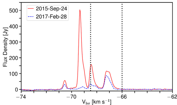
Figure 1. Selected spectra of the 6.7 GHz methanol masers associated with G323.46–0.08, observation taken on: 2015 September 24 (solid red line) and 2017 February 28. The vertical (dotted) lines, at -68.5 and -66.0 \text{km s}^{-1} , represent the velocity range in which 6.7 GHz methanol masers, with S_{\text{peak}} = 15.2 Jy, were previously reported by Green et al. (2012a).
