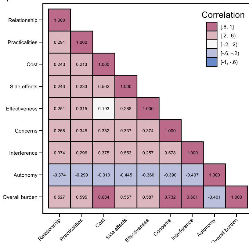
Fig. 2. The Spearman correlation between the themes of the LMQ-3 scale.
