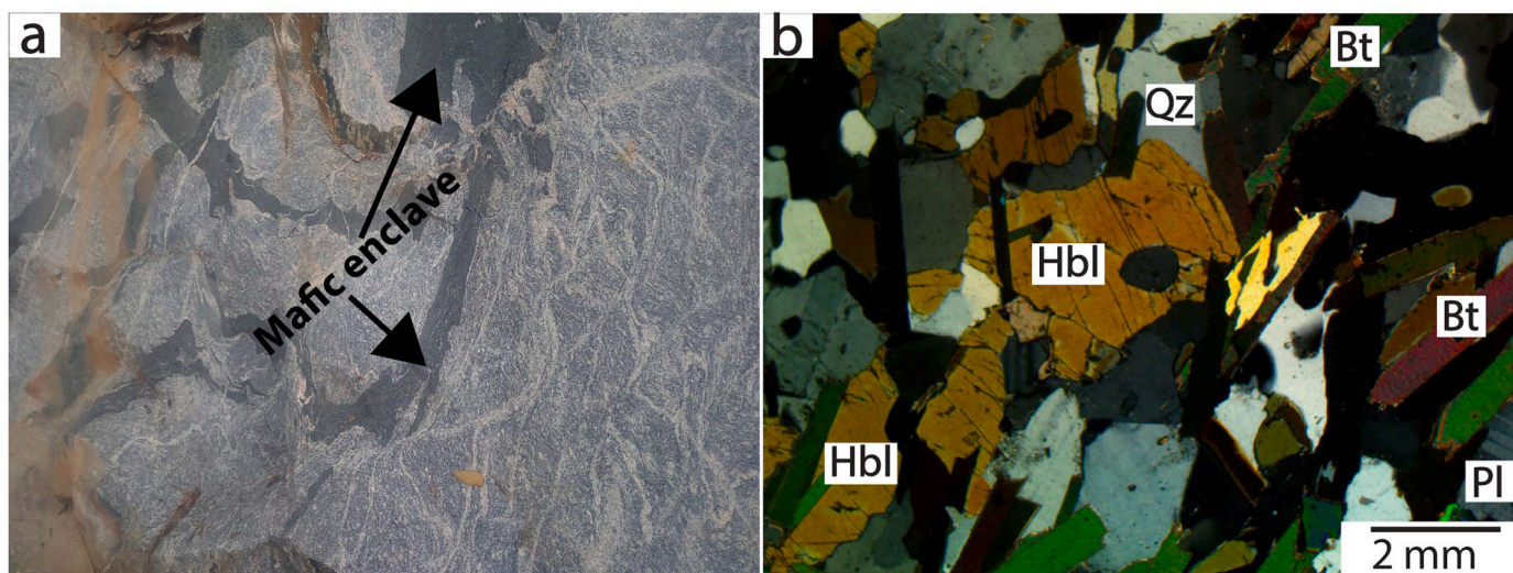
Fig. 5. (a) Field photo of mafic enclaves and (b) photomicrograph of mafic enclave, under cross polars.
