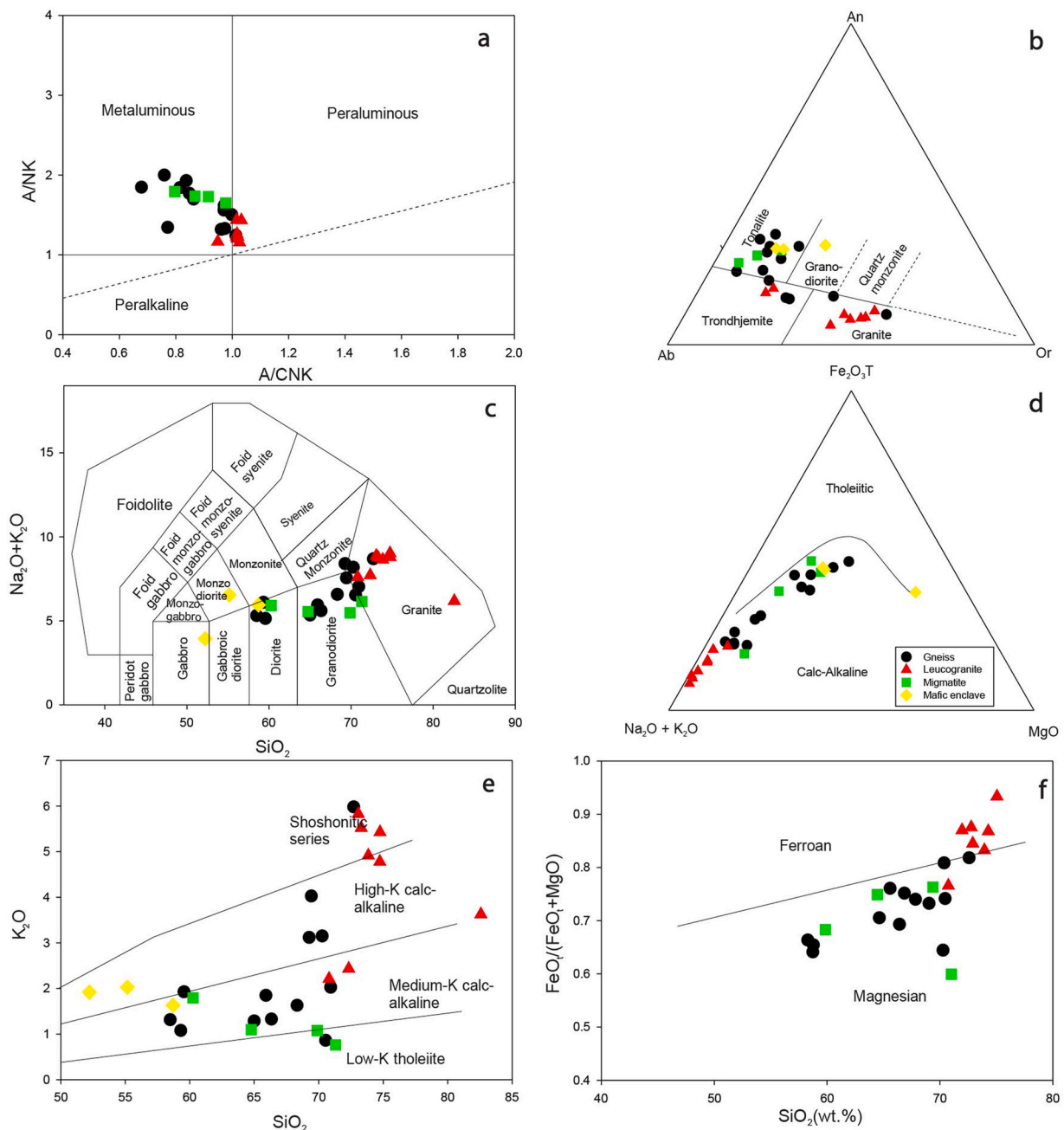
Fig. 9. Major element classification diagrams of the Suhum Basin granitoid complex (a) Plot of A/CNK (molar \text{Al}_2\text{O}_3/(\text{CaO} + \text{Na}_2\text{O} + \text{K}_2\text{O}) ) vs. ANK (molar \text{Al}_2\text{O}_3/(\text{Na}_2\text{O} + \text{K}_2\text{O}) ) (Maniar and Piccoli, 1989); (b) Or-Ab-An ternary diagram (O'Connor, 1965); (c) Total alkalis vs silica (TAS) (Middlemost, 1994); (d) AFM diagram (Irvine and Baragar, 1971); (e) \text{K}_2\text{O} vs. \text{SiO}_2 diagram (after Peccerillo and Taylor, 1976); and (f) \text{SiO}_2 vs. \text{FeO}_t/(\text{FeO}_t + \text{MgO}) diagram (after Frost and Frost, 2008).
