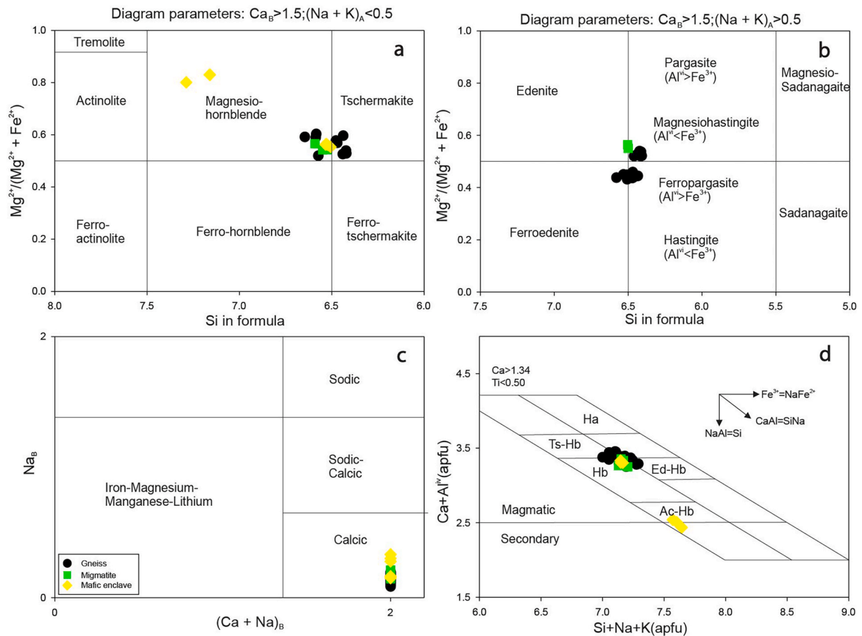
Fig. 8. (a) Amphibole classification diagram based on low (Na + K)_A content ( Leake et al., 1997 ); (b) Amphibole classification diagram based on higher (Na + K)_A content ( Leake et al., 1997 ); (c) The composition of the amphiboles ( Leake et al., 1997 ); and (d) Ca + Al^{IV} vs. Si + Na + K diagram ( Giret et al., 1980 ).
