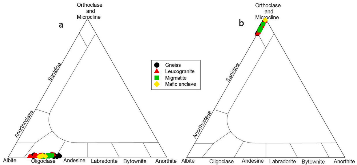
Fig. 7. Or-Ab-An ternary diagram of feldspar (after Howie et al., 1992 ) (a) plagioclase and (b) K-feldspar. Note: The samples from the granitoids complex of the Suhum Basin plot mainly as oligoclase, and microcline-orthoclase, respectively.
