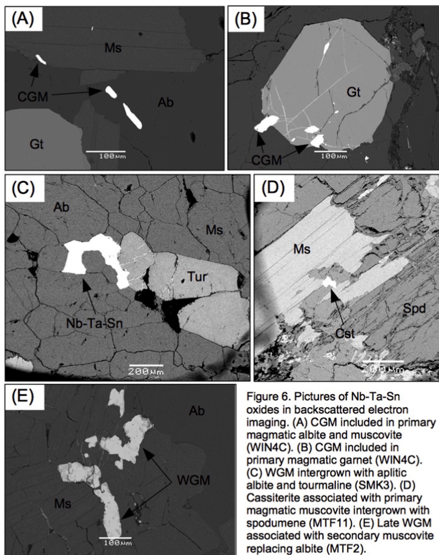
Fig. 6. Pictures of Nb-Ta-Sn oxides in backscattered electron imaging. (A) CGM included in primary magmatic albite and muscovite (WIN4C). (B) CGM included in primary magmatic garnet (WIN4C). (C) WGM intergrown with aplitic albite and tourmaline (SMK3). (D) Cassiterite associated with primary magmatic muscovite intergrown with spodumene (MTF11). (E) Late WGM associated with secondary muscovite replacing albite (MTF2).
