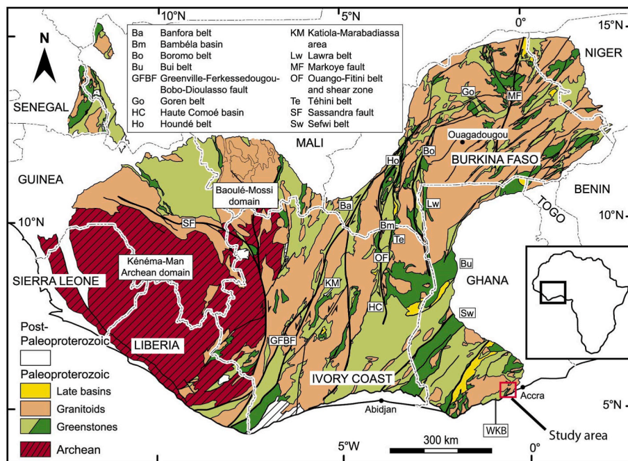
Fig. 1. The Leo Man Rise showing the Paleoproterozoic Birman Supergroup of Ghana. WKB = Winneba-Kibi belt. Modified after Milesi et al. (2004).
