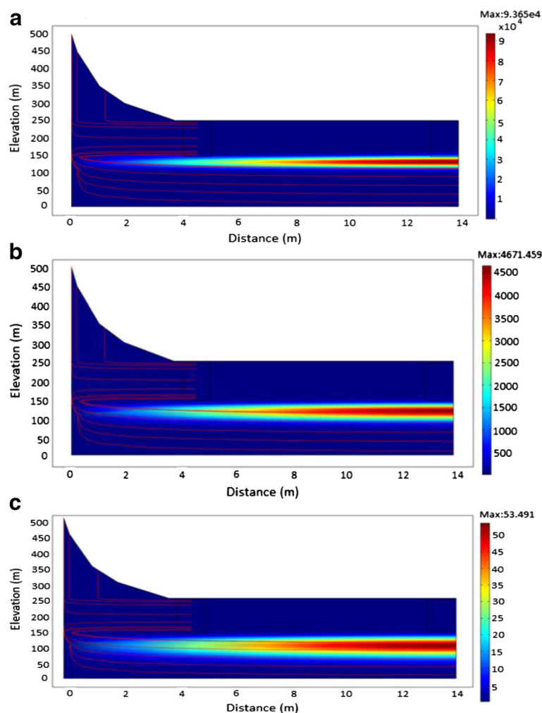
Figure 5 A plot showing the migration of ^{60}\text{Co} . a: From time of release to 250 years. b: From time of release to 500 years. c: From time of release to 1000 years
