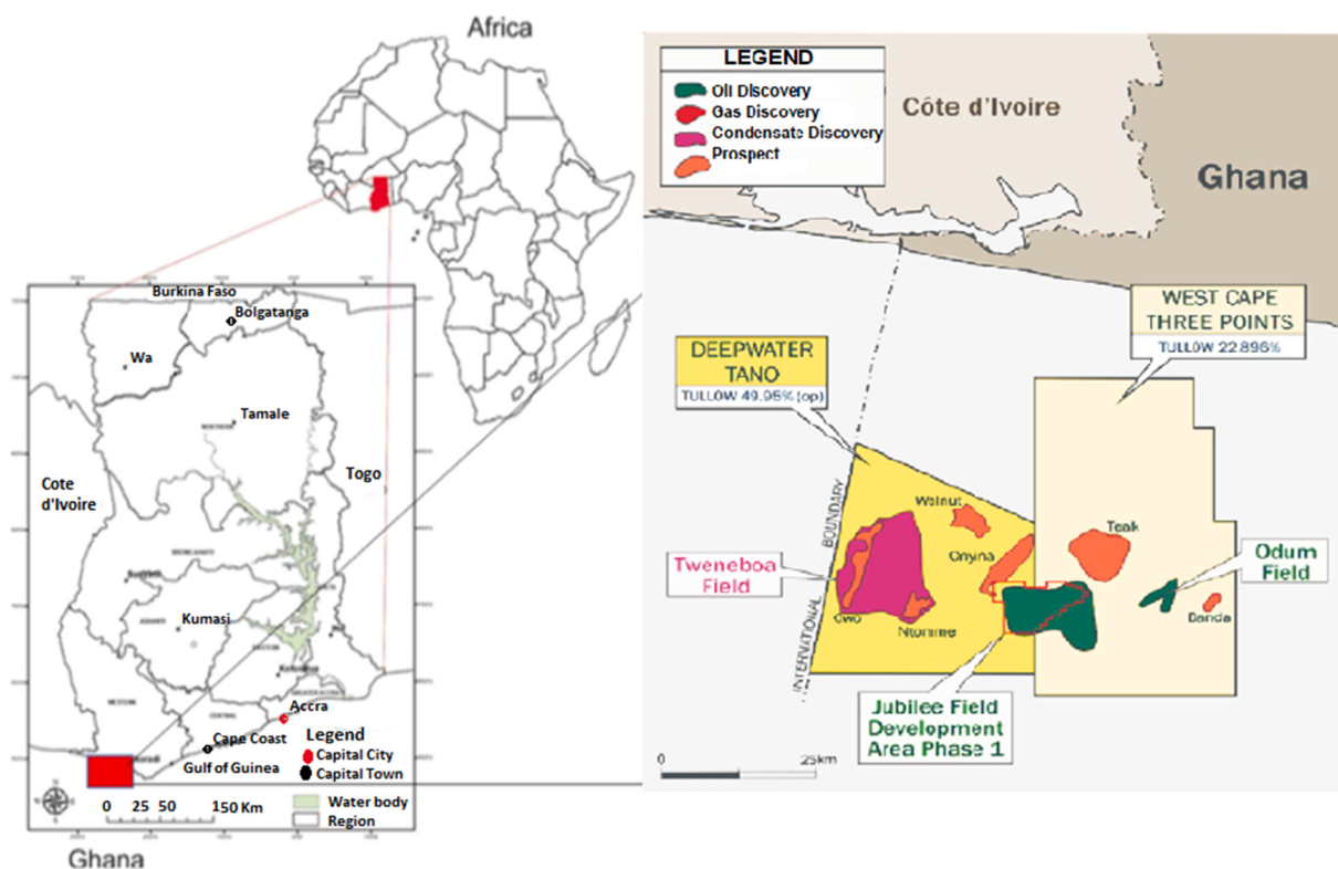
Fig. 1. Map of Ghana showing the Jubilee Oil Field where oil samples were collected [21].
