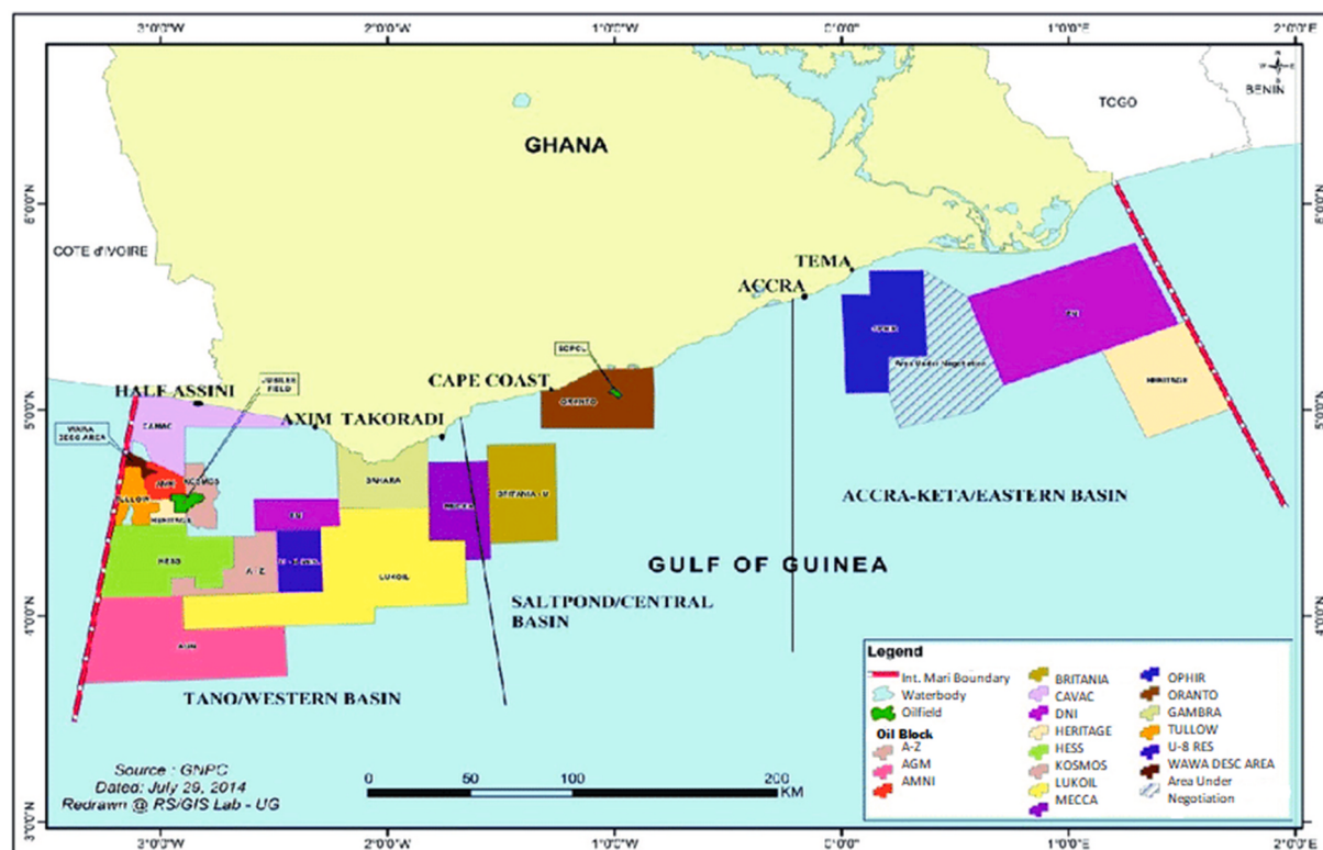
Fig. 2. Map Showing Three Distinct Oil Basins in Ghana where water samples were collected.
