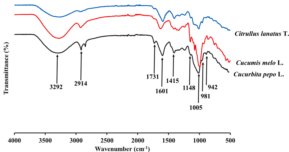
Fig. 2. FTIR of Cucurbitaceae pectin.
