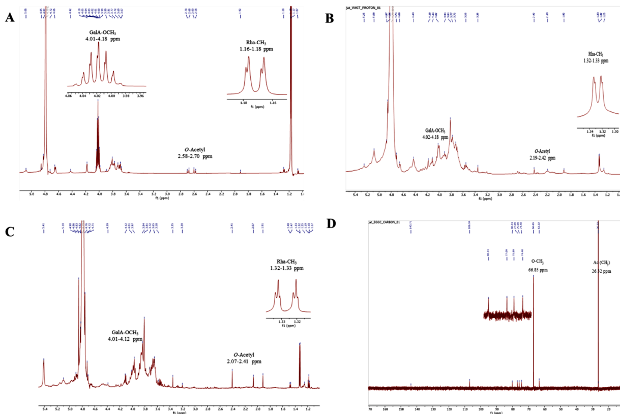
Fig. 3. ^1\text{H} NMR spectra of pectin from Cucumis melo L. (A), Citrullus lanatus T. (B), Cucurbita pepo L. (C), ^{13}\text{C} NMR spectra of Cucumis melo L. (D).
