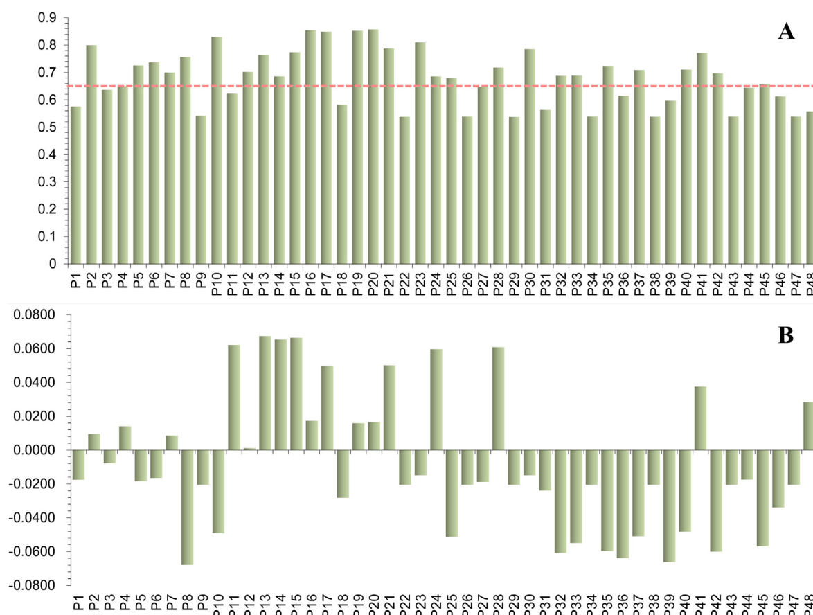
Fig. 4 The GCA and PLSR plots of the relationship between the GC–MS spectrum and the vasodilatory activities of EONJs (A) Grey correlation degree plot of each constituent to the vasodilatory efficacy (GCA); (B) Regression coefficient plot of each constituent to the vasodilatory efficacy (PLSR).
