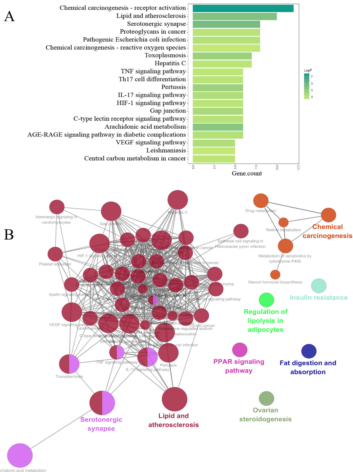
Fig. 10 KEGG pathway enrichment analysis (A) The bar chart on the top 20 significantly enriched KEGG pathway terms by RStudio; (B) The network diagram of KEGG pathway enrichment analysis by clueGO. (Each node indicates the enriched KEGG pathway term, the more significant the p -value is, the larger the node is; different colors represent different pathway groups, the bold font is treated as the pathway representation, and the line between nodes means the correlation among pathways).
