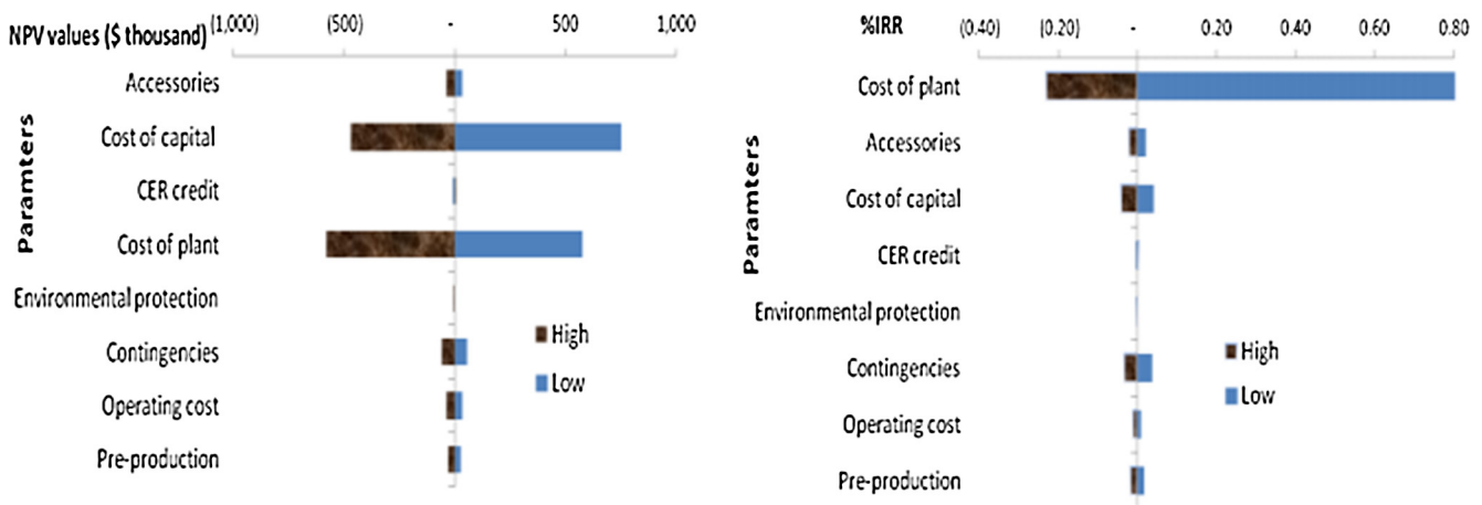
Figure 4 (a) NPV tornado chart – cooking option and (b) IRR tornado chart – cooking option.
