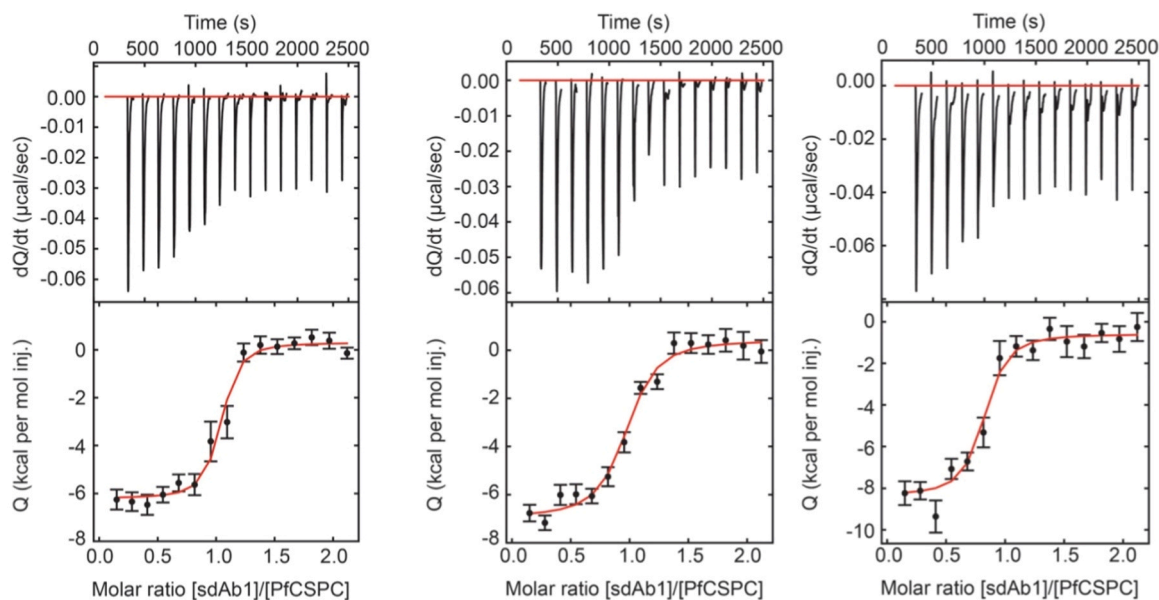
Fig. 6. ITC - ITC measurements at 25 °C for the binding of sdAbCSP1 to PfCSP-C. Each replicate measurement is shown. The top panels represent the thermograms in which the black lines depict the raw data. The bottom panels show the isotherms. The black dots display the experimental data points, and the red traces show the fit.
