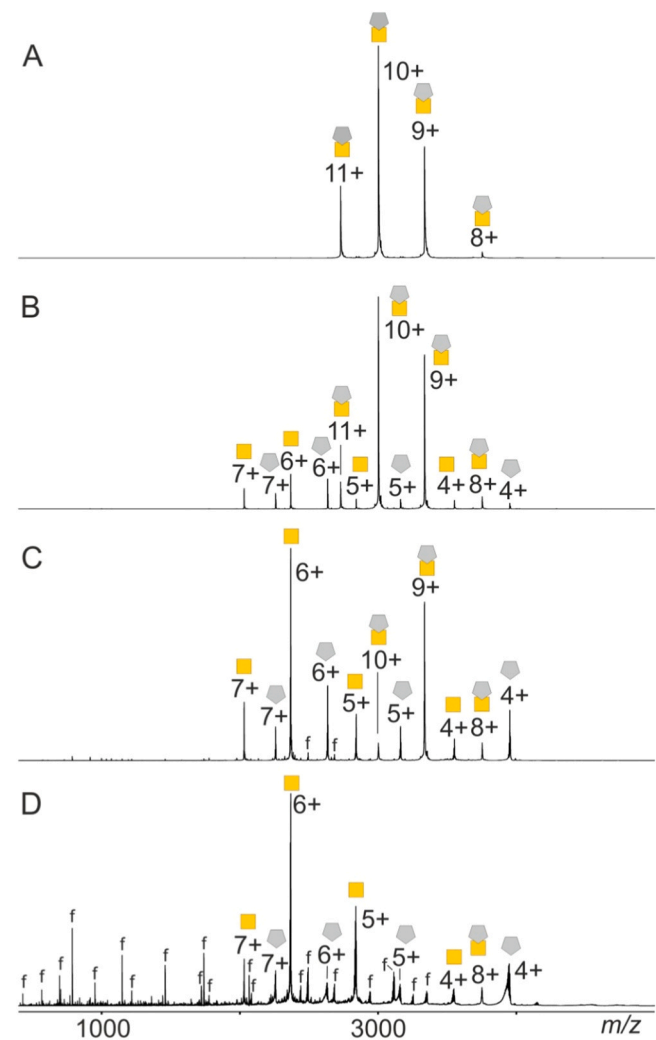
Fig. 5. Offline nanoESI mass spectra of sdAbCSP1 – PfCSP-Cext complex dissociation at different collision cell voltage difference settings. A , \Delta CV 10 V. B , \Delta CV 40 V. C , \Delta CV 70 V. D , \Delta CV 100 V. Molar ratio of sdAbCSP1: PfCSP-Cext = 1: 3.4. Ion signals are labeled with charge states. Gold-colored square & gray-colored pentagon, sdAbCSP1 – PfCSP-Cext complex; Gold-colored square, PfCSP-Cext; Gray-colored pentagon, sdAbCSP1; f: fragments. The quadrupole was set to block transmission of ions with m/z < 2400 . Solvent: 200 mM ammonium acetate, pH 6.7. For ion signal intensities, see Tables S13, S14, and S15.
