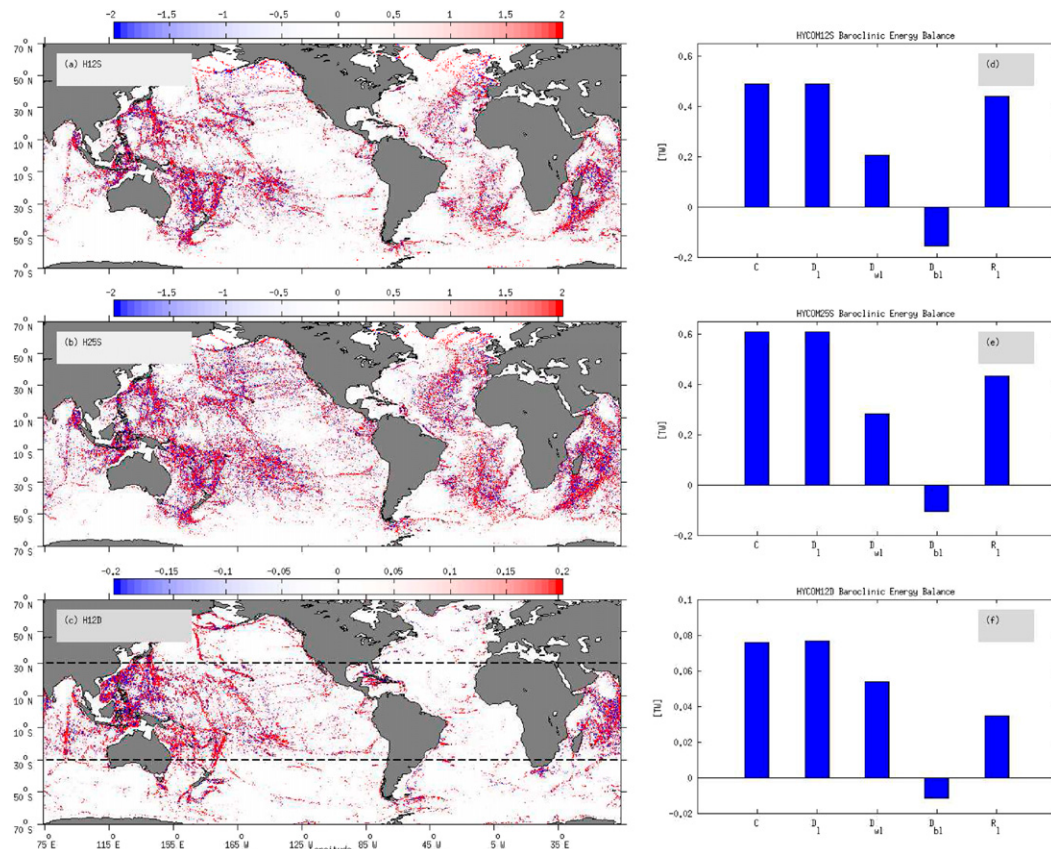
FIG. 2. (left) Barotropic to baroclinic energy conversion ( \text{mW m}^{-2} ) for (a) HYCOM12S (b) HYCOM25S, and (c) HYCOM12D. (right) Baroclinic energy balance analysis for corresponding resolutions in the left panels, with barotropic to baroclinic conversion C , low-mode dissipation D_l , topographic wave drag dissipation D_{wl} , dissipation due to bottom friction D_{bl} , and residual term R_l .
