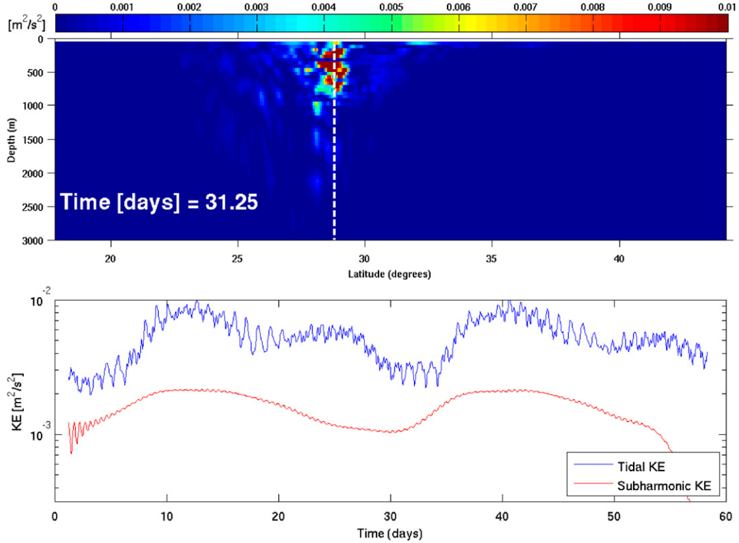
FIG. 5. (a) Snapshot of the subharmonic baroclinic kinetic energy density ( u^2 + v^2 ) from the vertical section in Fig. 4b, computed from HYCOM12S. (b) Temporal variation of vertically averaged subharmonic kinetic energy density from the vertical section in (a).
