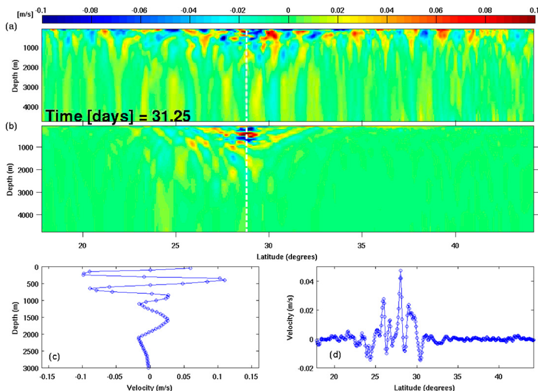
FIG. 4. (a) Snapshot of semidiurnal tidal signal of meridional baroclinic velocity from HYCOM12S close to location MP3 (29.1°N, 163.5°W) around Hawaii. (b) As in (a), but after bandpassing around the subharmonic frequency band. Observe the high vertical wavenumber structure in the upper ocean around the CL. (c) A vertical profile through the M_2 critical latitude ( \sim 28.8^\circ ) from (b), showing the vertical scale of the subharmonic signal. (d) A horizontal slice of (b) through 1000-m depth, showing the horizontal scale of the subharmonic signal in the critical latitude band ( 25^\circ – 30^\circ N).
