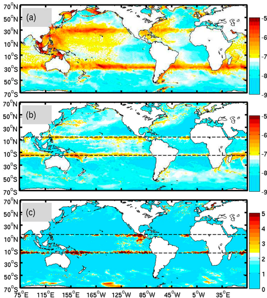
FIG. 7. As in Fig. 6, but for HYCOM12D.
