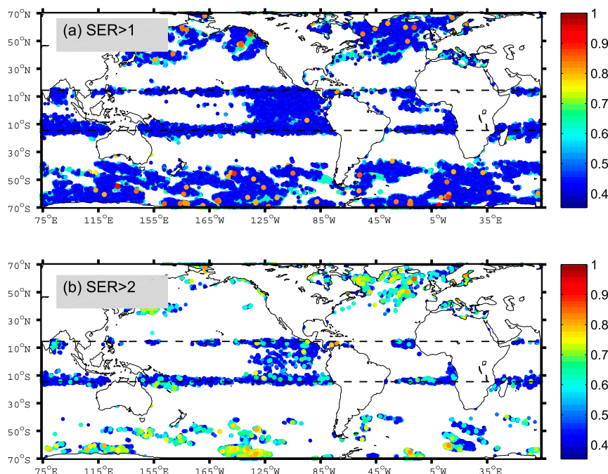
FIG. 9. As in Fig. 8, but for HYCOM12D.
