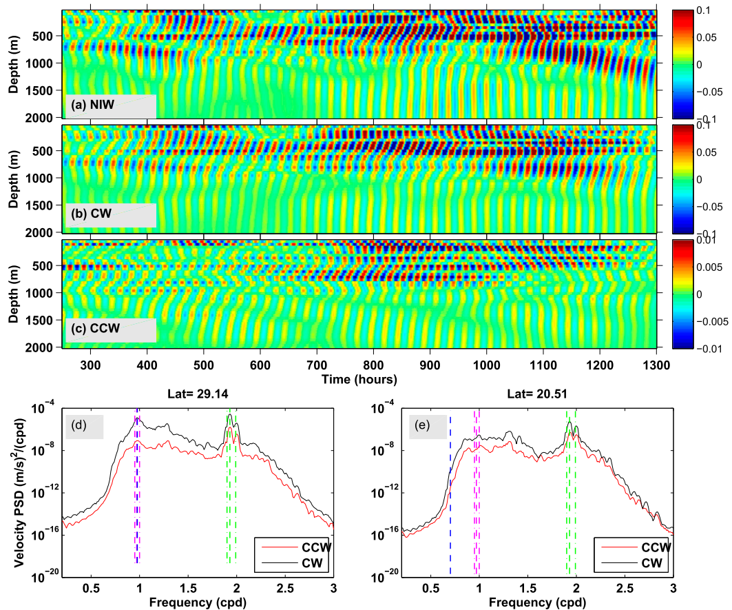
FIG. 3. (a)–(c) Time series of northward velocity ( \text{m s}^{-1} ) from HYCOM12S near location MP3 ( 29.1^{\circ}\text{N} , 163.5^{\circ}\text{W} ) around Hawaii showing the bandpassed signals at the (a) subharmonic near-inertial frequency band (NIW), and the component of the subharmonic signal rotating (b) CW and (c) CCW. (d) The PSD of the signals in (b) and (c), and (e) the PSD at location ( 20.5^{\circ}\text{N} , 163.5^{\circ}\text{W} ). The green and magenta dashed lines indicate the frequencies of the semidiurnal tidal constituents and their subharmonics, respectively, and the blue dashed line show the local inertial frequency.
