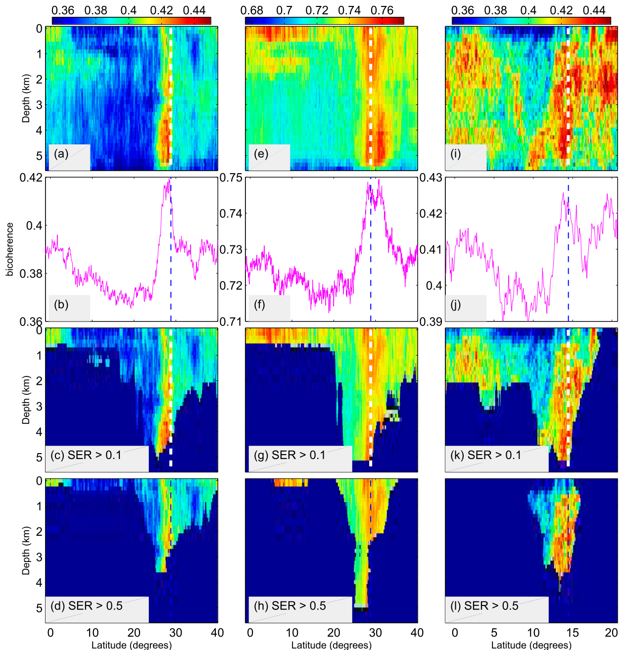
FIG. 10. (a) Variation in depth and latitude of zonally averaged bicoherence for HYCOM12S. (b) Vertically averaged bicoherence values in (a), showing a drop-off in intensity of bicoherence away from the critical latitude. The dashed vertical lines indicate the position of the M_2 critical latitude. (c),(d) As in (a), but with zonally averaged SER > 0.1 and SER > 0.5, respectively. (e)–(h) As in (a)–(d), but for HYCOM25S. (i)–(l) As in (a)–(d), but for HYCOM12D.
