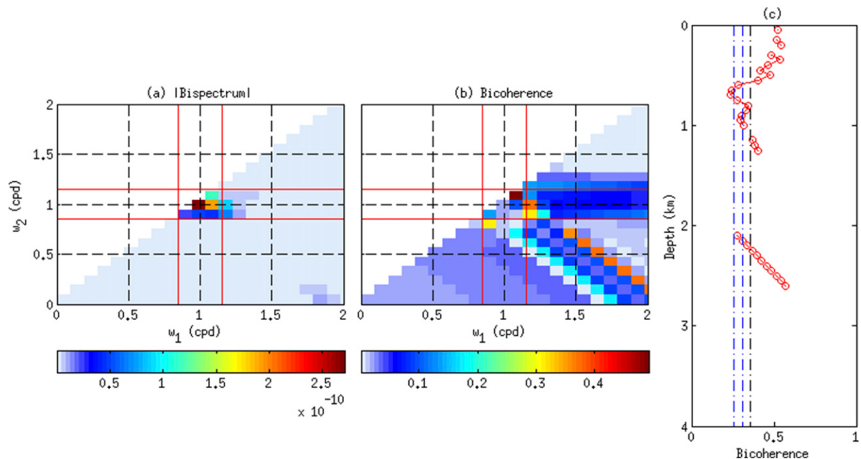
FIG. A1. Example bispectral calculation from HYCOM12S at location (29.14°N, 163.5°W), depicting the (a) bispectrum and (b) bicoherence at about 500-m depth, and (c) significant bicoherence values at each vertical level. The vertical dashed lines in (c) show the value at the 80%, 90%, and 95% significance levels.
