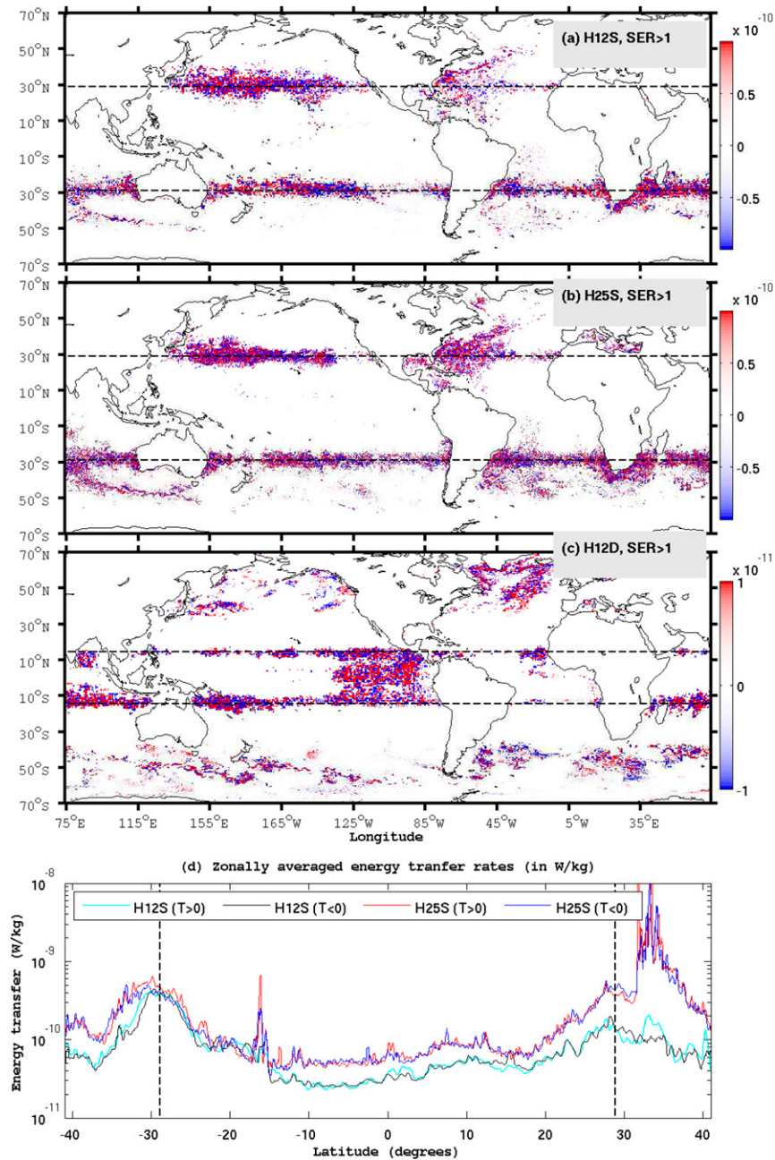
FIG. 12. Vertically integrated global distribution of energy transfer rates ( \text{W kg}^{-1} ) between low-mode tides and subharmonic signals for (a) HYCOM12S, (b) HYCOM25S, and (c) HYCOM12D. (d) Zonally averaged energy transfer rates from HYCOM12S (H12S) and HYCOM25S (H25S), showing that the positive and negative transfers have about the same magnitude, leading to a negligible net energy transfer. “T” is used to denote the sign of energy transfer.
