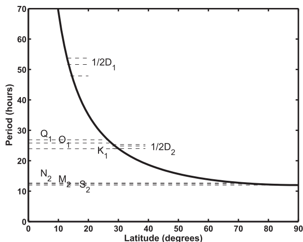
FIG. 1. Periods of the diurnal ( K_1 , O_1 , Q_1 ; D_1 collectively) and semidiurnal ( M_2 , S_2 , N_2 ; D_2 collectively) tides as well as periods of their half-frequency subharmonics [ (1/2)D_1 and (1/2)D_2 , respectively]. The solid curve shows the local period of inertial oscillations f as a function of latitude. Lines to the left of f are for D_2 and D_1 ; those to the right are for (1/2)D_2 and (1/2)D_1 .
