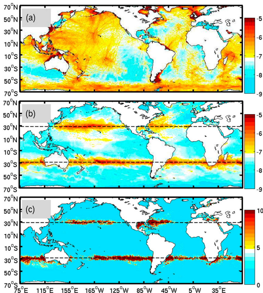
FIG. 6. Global distribution of bandpassed and vertically integrated PSD from HYCOM12S for the (a) semidiurnal band, (b) subharmonic band, and (c) SER. Note that the maximum SER in (c) is about 400.
