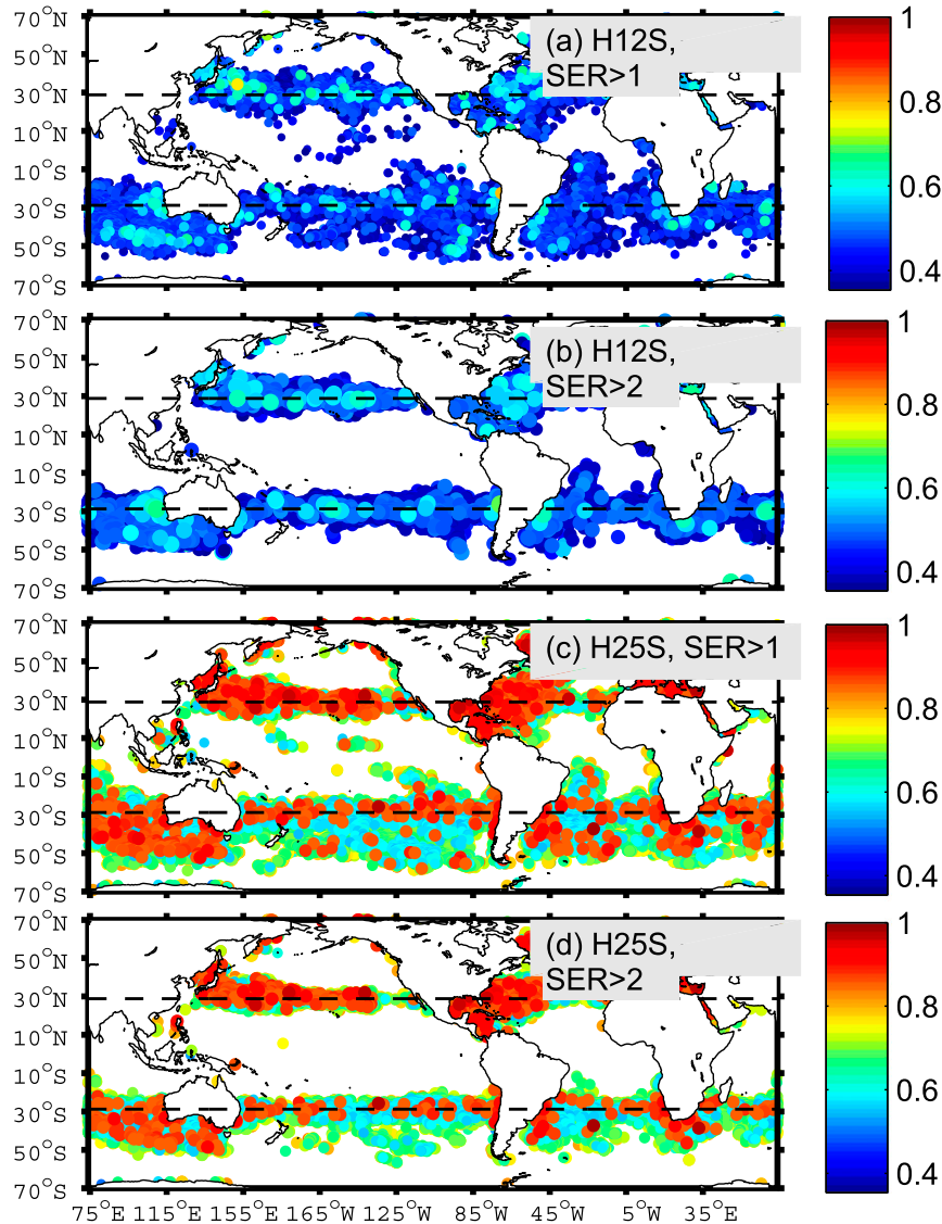
FIG. 8. Global distribution of vertically averaged bicoherence for (a) HYCOM12S ( SER > 1 ), (b) HYCOM12S ( SER > 2 ), (c) HYCOM25S ( SER > 1 ), and (d) HYCOM25S ( SER > 2 ). The plots display significant bicoherence values at the 95% significance level ( b_{95\%} = 0.35 for HYCOM12S and 0.50 for HYCOM25S), and every sixth grid point is plotted.
