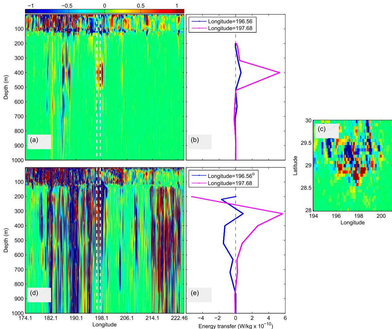
FIG. 11. Energy transfer rates from HYCOM12S (a) at a zonal section along latitude 29.14^{\circ}\text{E} ( \times 10^{-10} \text{ W kg}^{-1} ), (b) in a vertical profile near location MP3 (blue curve) and just to the east of MP3 (magenta curve), and (c) at a depth of about 400 m near MP3. (d),(e) As in (a) and (b), but for HYCOM25S. The white dashed lines in (a) and (d) show the positions of profiles given by the blue and magenta curves in (b) and (e).
