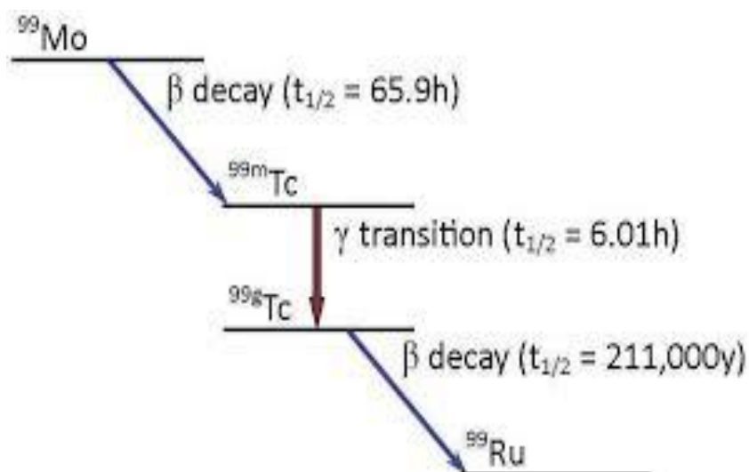
Fig. 2.1: Decay scheme for ^{99}\text{Mo}
