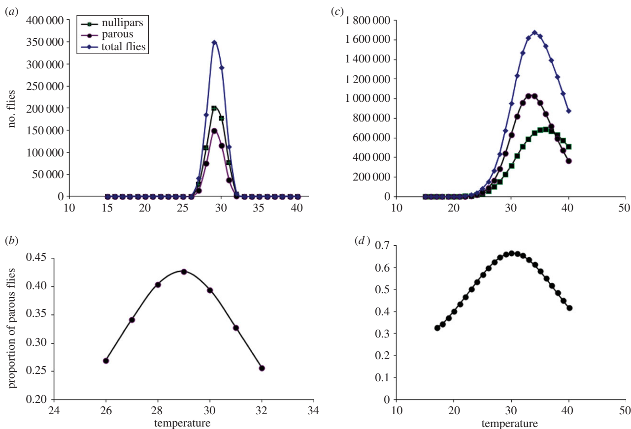
Figure 4. Output of blackfly population models with parameters for Liberia (forest) ( a,b ) and Ghana (savannah) ( c,d ). ( a,c ) Equilibrium densities of total numbers of flies (diamonds), nulliparous flies (squares) and parous flies (circles) at different temperatures ( ^{\circ}\text{C} ). ( b,d ) Proportions of parous flies at different temperatures ( ^{\circ}\text{C} ). (Online version in colour.)
