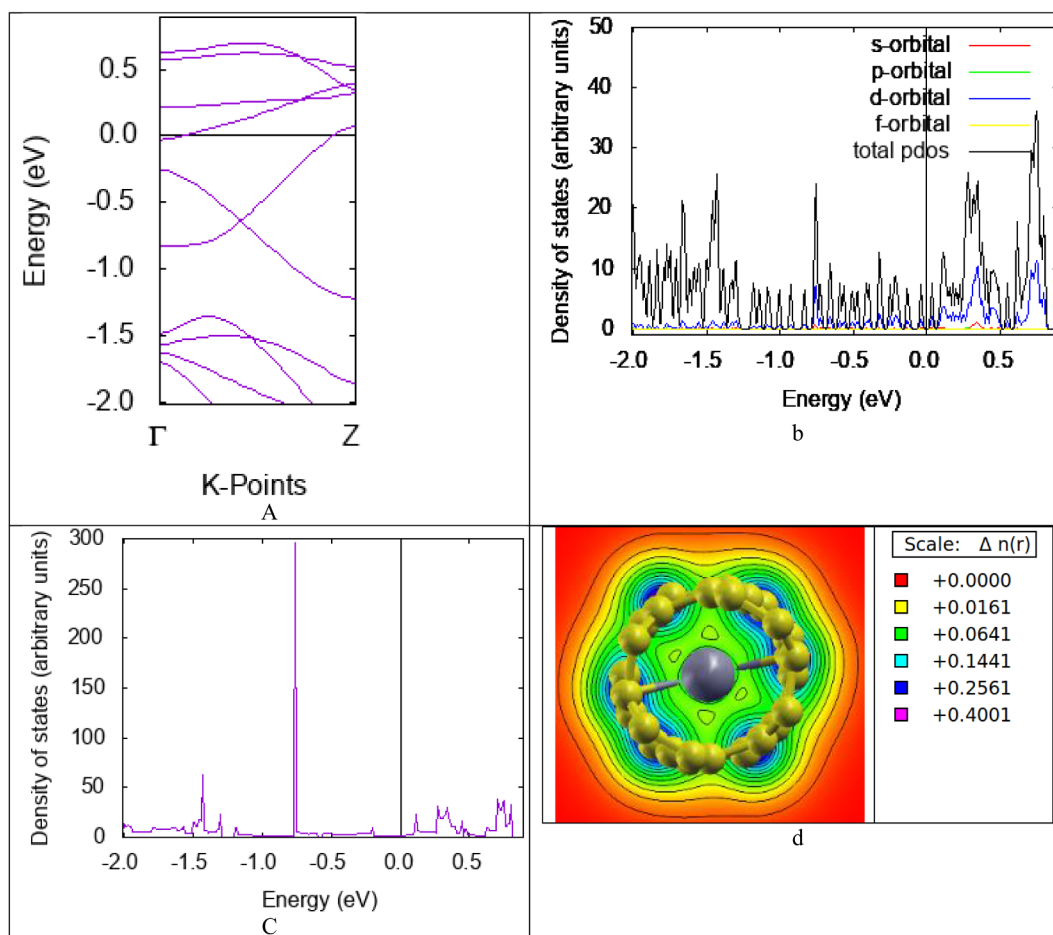
Fig. 4. Where a- Band structure of (4,2) CNT with Ti interacting at site 3, b- PDOS of (4,2) CNT with Ti interacting at Site 3, c- DOS of (4,2) CNT with Ti interacting at Site 3, d- Charge density of (4,2) CNT with Ti interacting at Site 3.
