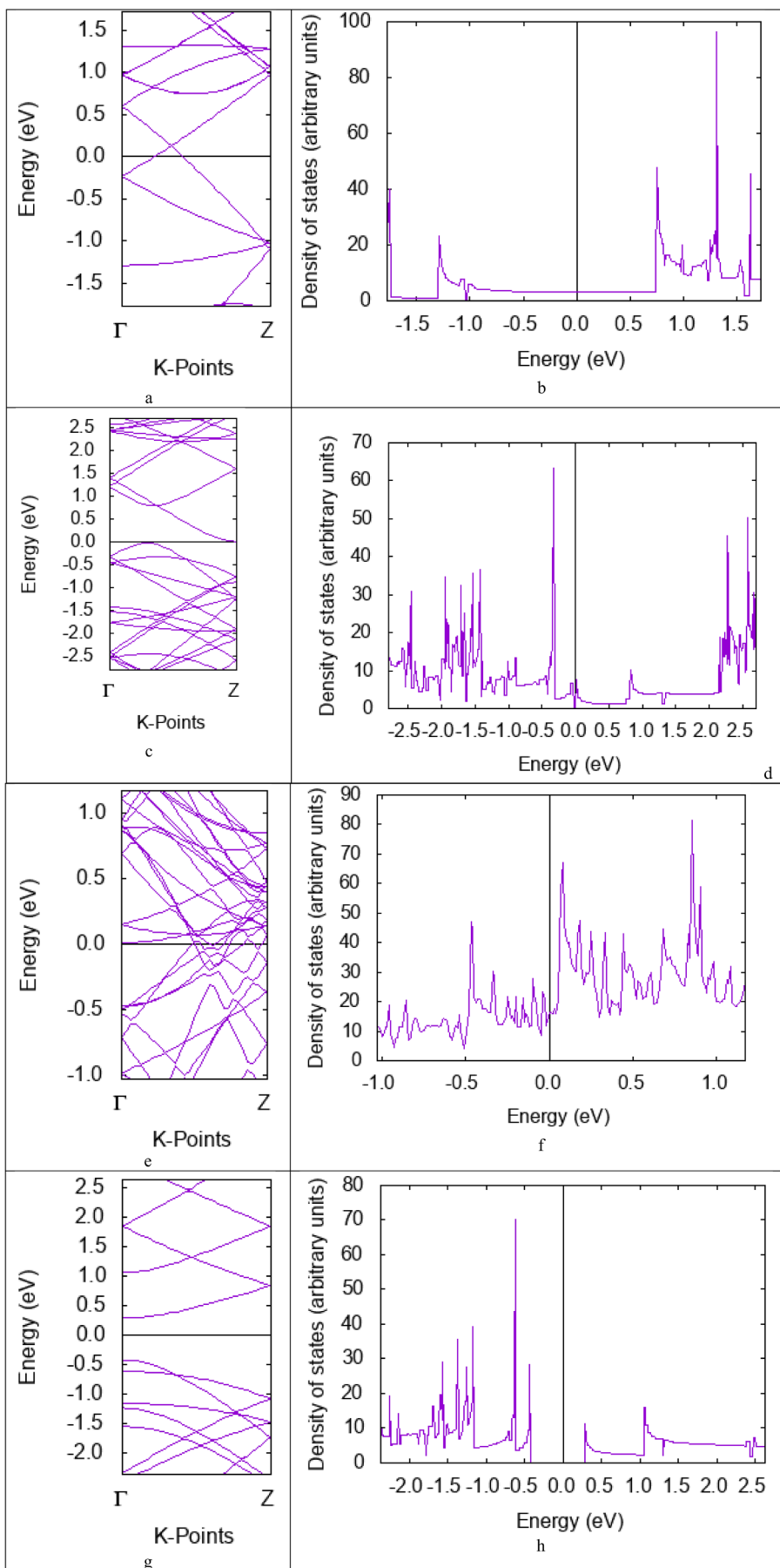
Fig. 2. a- Band structure of a pristine (3,3) CNT, b- DOS of a pristine (3,3) CNT, c- Band structure of a pristine (4,2) CNT, d- DOS of a pristine (4,2) CNT, e- Band structure of a pristine (5,1) CNT, f- DOS of a pristine (5,1) CNT, g- Band structure of a pristine (6,0) CNT, h- DOS of a pristine (6,0) CNT.
