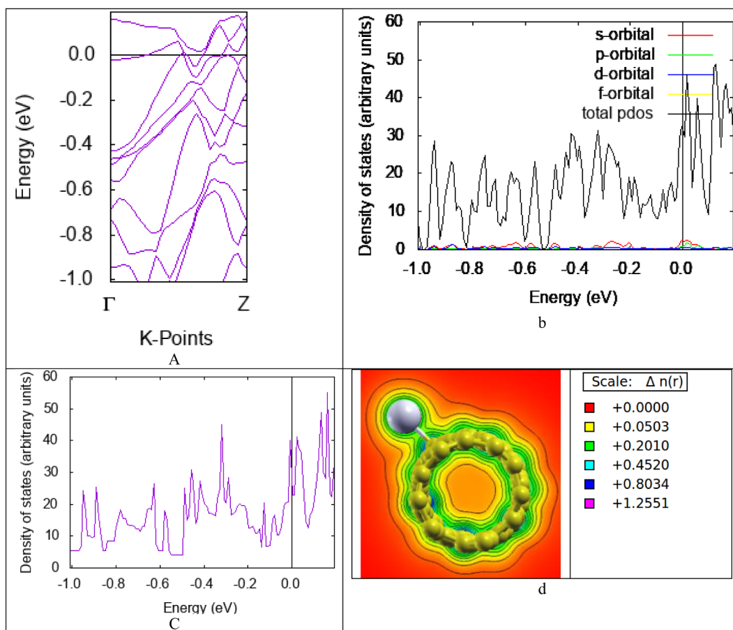
Fig. 5. Where a- Band structure of (5,1) CNT with Pd adsorbed at Site 1, b- Projected DOS of (5,1) CNT with Pd adsorbed at Site 1, c- DOS of (5,1) CNT with Pd adsorbed at Site 1, d- Charge density of (5,1) CNT with Pd adsorbed at Site 1.
