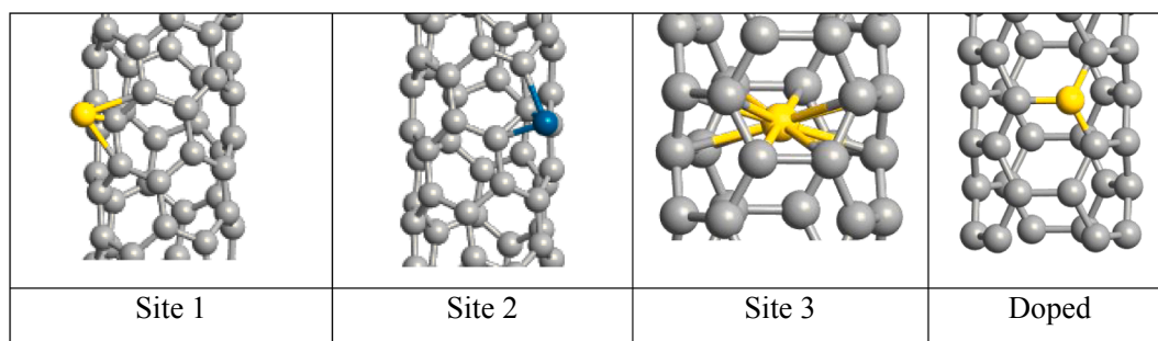
Fig. 1. Different interaction sites for Gold (yellow) and Palladium (blue) metal atoms on a (5,1) CNT and (3,3) CNT. (For interpretation of the references to colour in this figure legend, the reader is referred to the web version of this article.)
