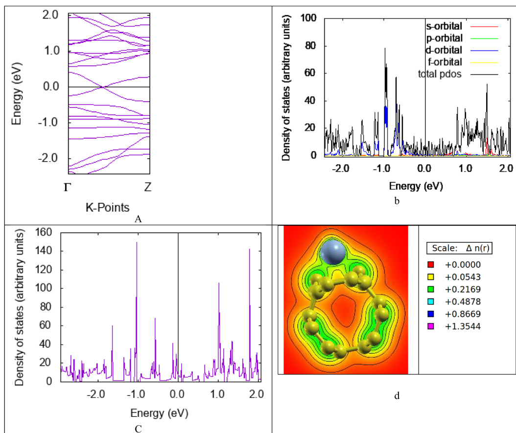
Fig. 3. Where a- Band structure of a (3,3) CNT with Ni adsorbed at Site 2, b- PDOS of a (3,3) CNT with Ni adsorbed at Site 2, c- DOS of a (3,3) CNT with Ni adsorbed at Site 2, d- Charge density plot for a (3,3) CNT with Ni adsorbed at Site 2.
