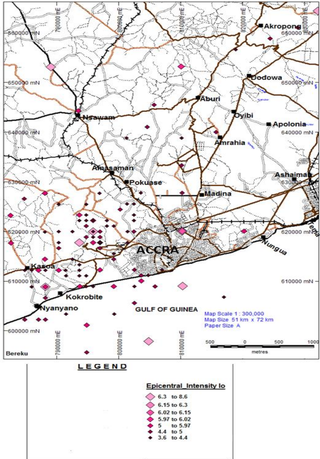
Fig. 5.2: A Plot of the Epicentral Intensity Map of the Study Area
