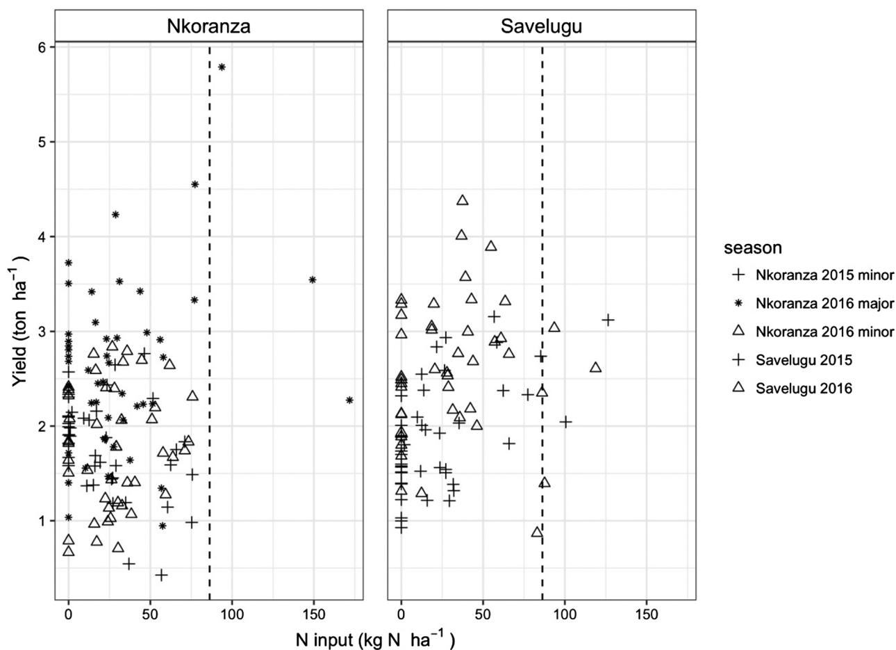
Fig. 6. Yield versus N input for Nkoranza and Savelugu for the 2015 and 2016 seasons. Dashed lines represent the recommended N input.
