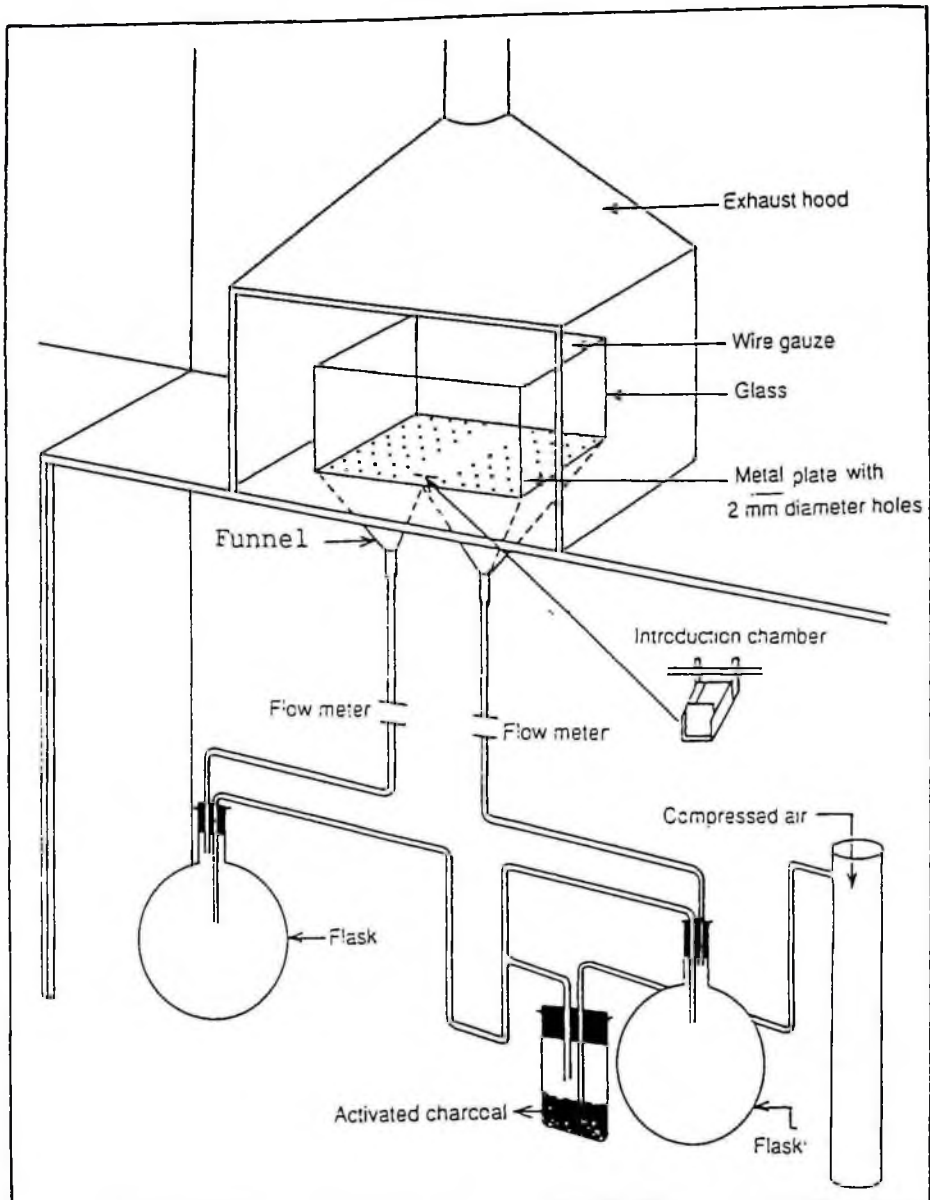
Figure 4. Diagram of the olfactometric aggregation bioassay system
