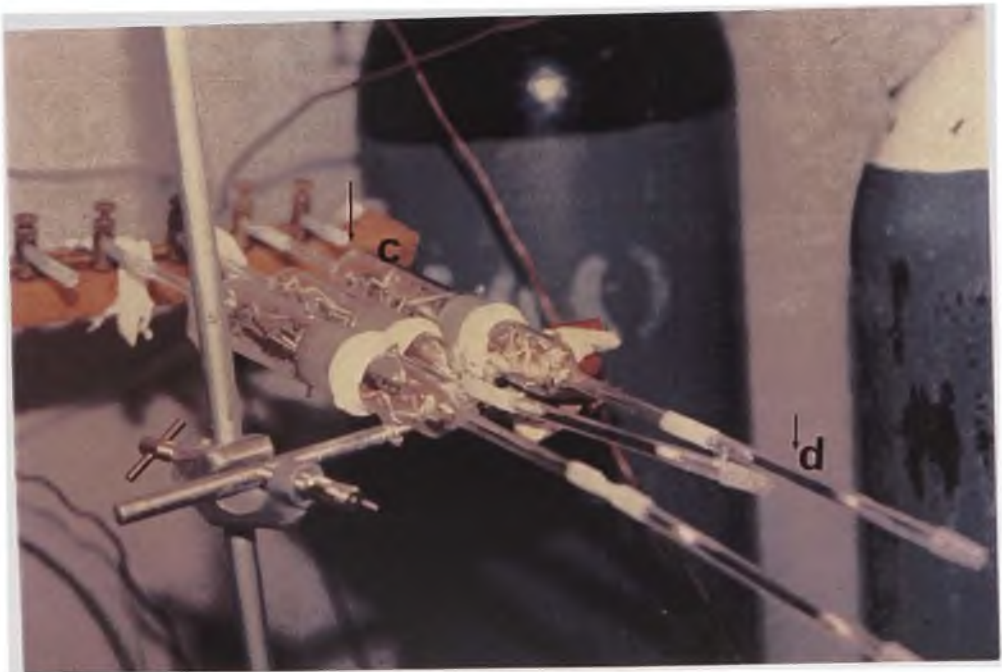
B. Volatile collection system (B-1) showing connected to it a) three-neck round bottomed flask containing mature S. gregaria b) quickfit trapping chambers, and the medical air source cylinders; quickfit chambers (c) with connected charcoal traps (d) (B-2)
