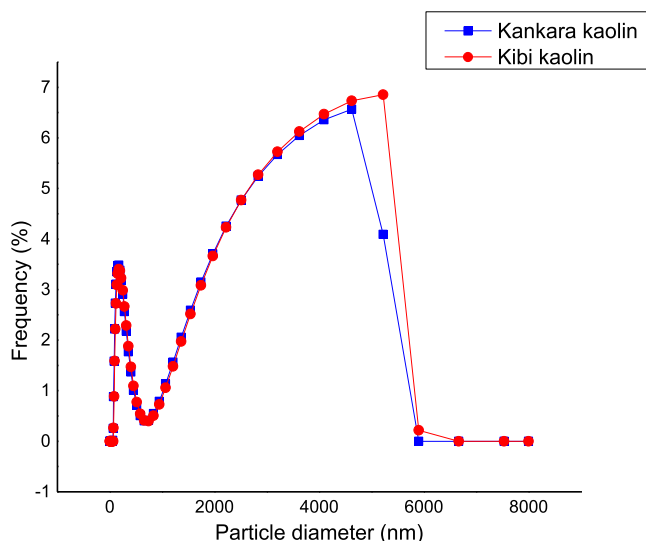
Fig. 1. Particle size distributions of Kankara and Kibi kaolin.
