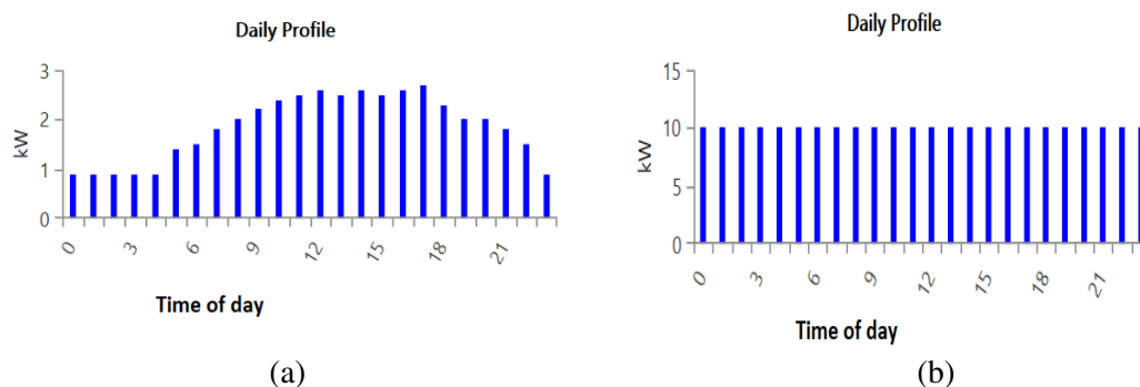
Figure 2. (a) load profile of Hospital and tourism centre (b) Telecommunication base station
