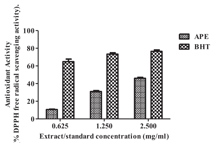
Fig. 2. DPPH free radical scavenging activity of varying concentrations of APE and the standard BHT. Results are means \pm S.E.M. of n = 3 . APE = A. polycarpa aqueous stem bark extract; BHT = butylated hydroxytoluene.
