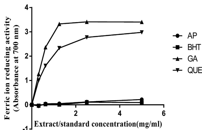
Fig. 3. The ferric ion reducing activity of varying concentrations of quercetin, Gallic acid, butylated hydroxytoluene (BHT) and A. polycarpa aqueous stem bark extract (APE). Results are means \pm S.E.M. of n = 3 .
