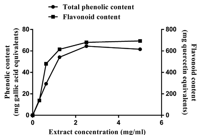
Fig. 1. Total phenolic and flavonoid contents of increasing concentration of APE. Values are means \pm S.E.M. of n = 3 . APE = A. polycarpa aqueous stem bark extract.
