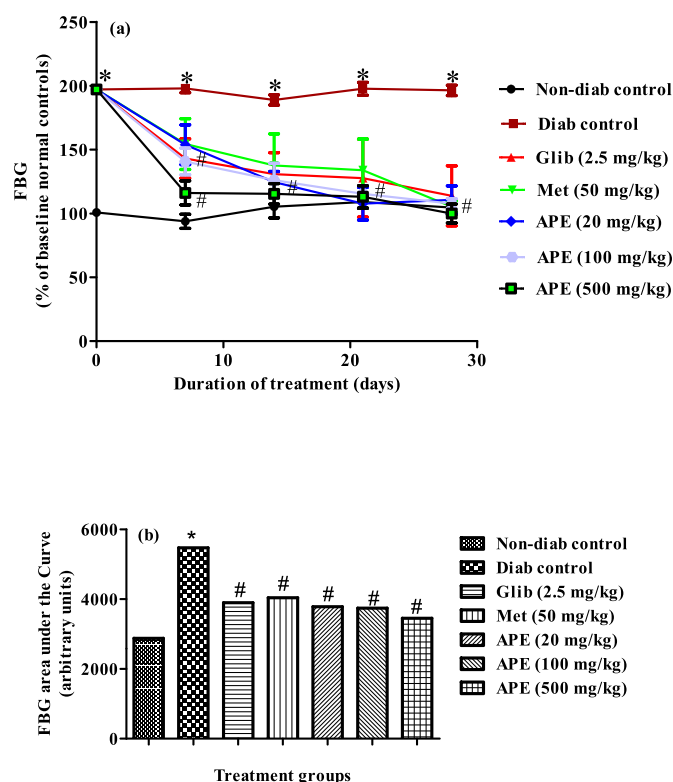
Fig. 4. Effect of APE and standard drugs on FBG levels; (a): line graph and (b): area under the curves (AUC). Values are percentages of baseline normoglycaemic control FBG ( 4.3 \pm 0.1 mmol/L). Results are means \pm S.E.M. of n = 5 . Glib = glibenclamide; Met = metformin; APE = A. polycarpa aqueous stem bark extract; FBG = fasting blood glucose. *Value significantly different from normoglycaemic control ( p < 0.05 ). #Value significantly different from diabetic control ( p < 0.05 ).
