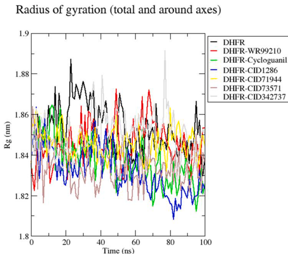
Fig. 7. Radius of Gyration plots of the unbound Pf DHFR (black) and the Pf DHFR-ligand complexes after the 100 ns MD. Rg plots of DHFR-WR99210, DHFR-Cycloguanil, DHFR-CID1286, DHFR-CID71944, and DHFR-CID73571 DHFR-CID342737, are shown in red, green, blue, yellow, brown and gray respectively.
