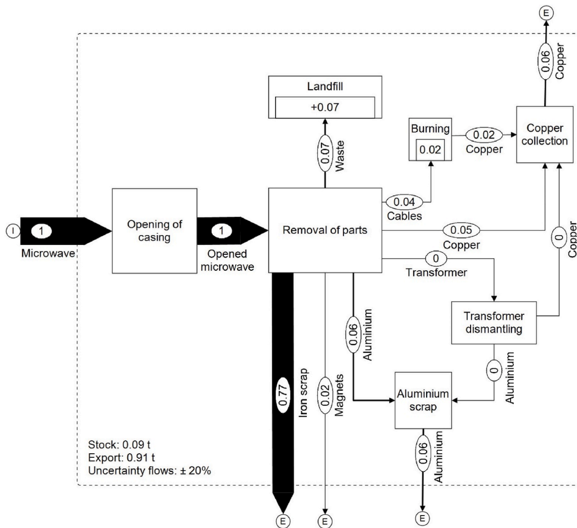
Fig. 8. Process flow of microwave dismantling in the informal sector.
