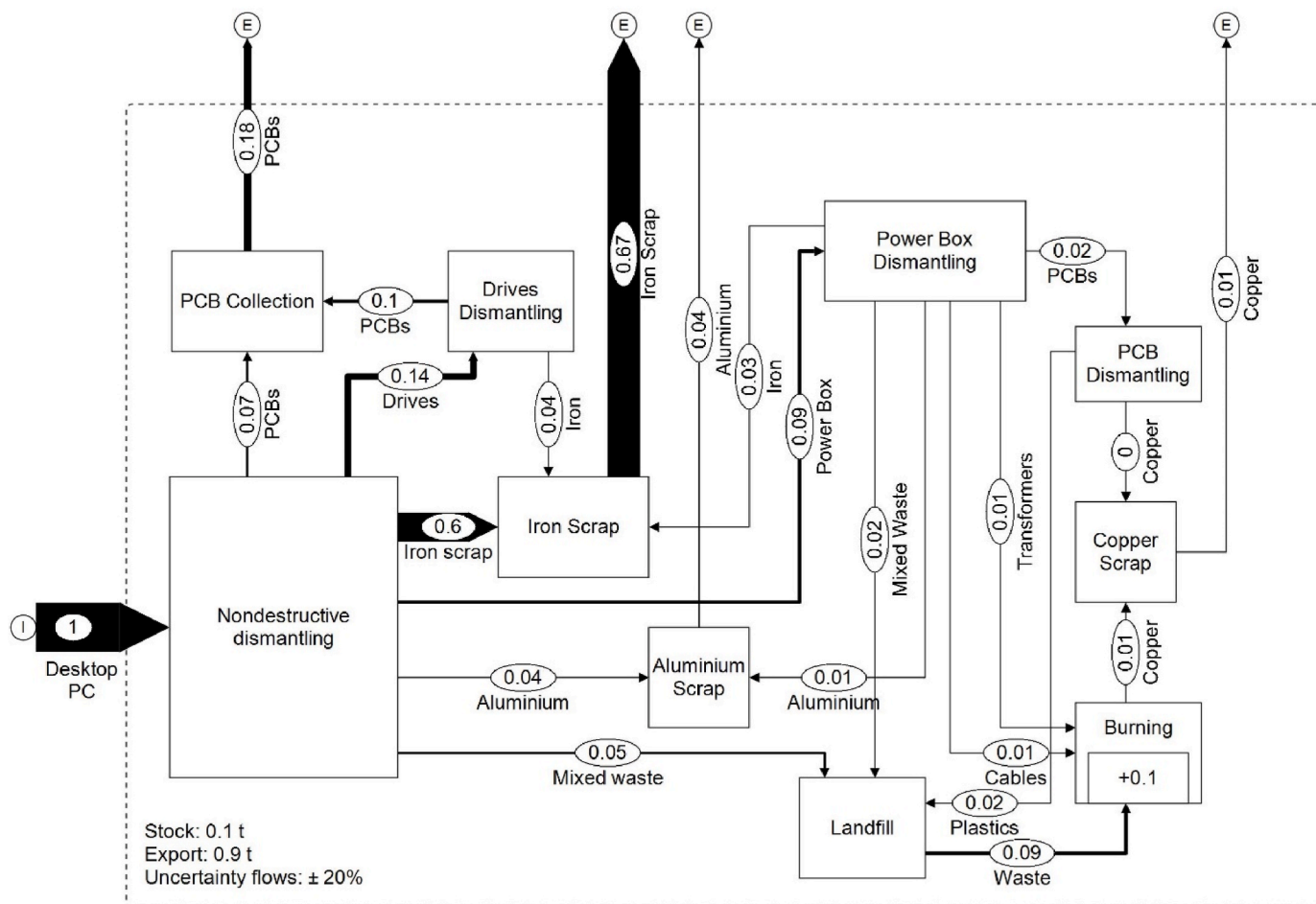
Fig. 3. Process flow in informal sector of desktop PC dismantling. Casing, power boxes and drives are dismantled in independently operating workshops.
