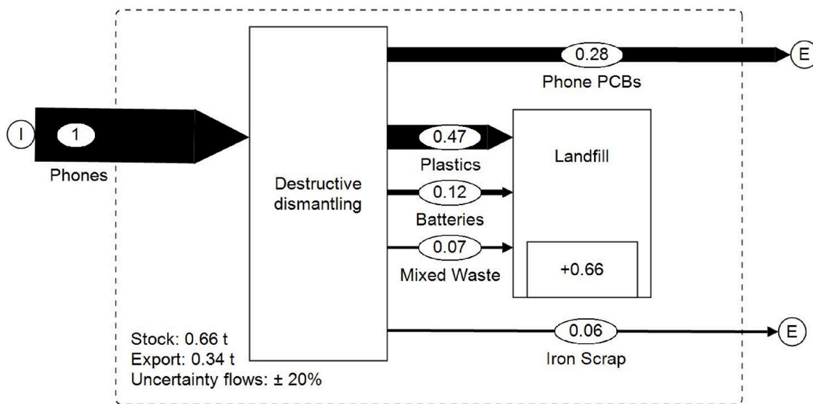
Fig. 5. Process flow of mobile phone dismantling in the informal sector.
