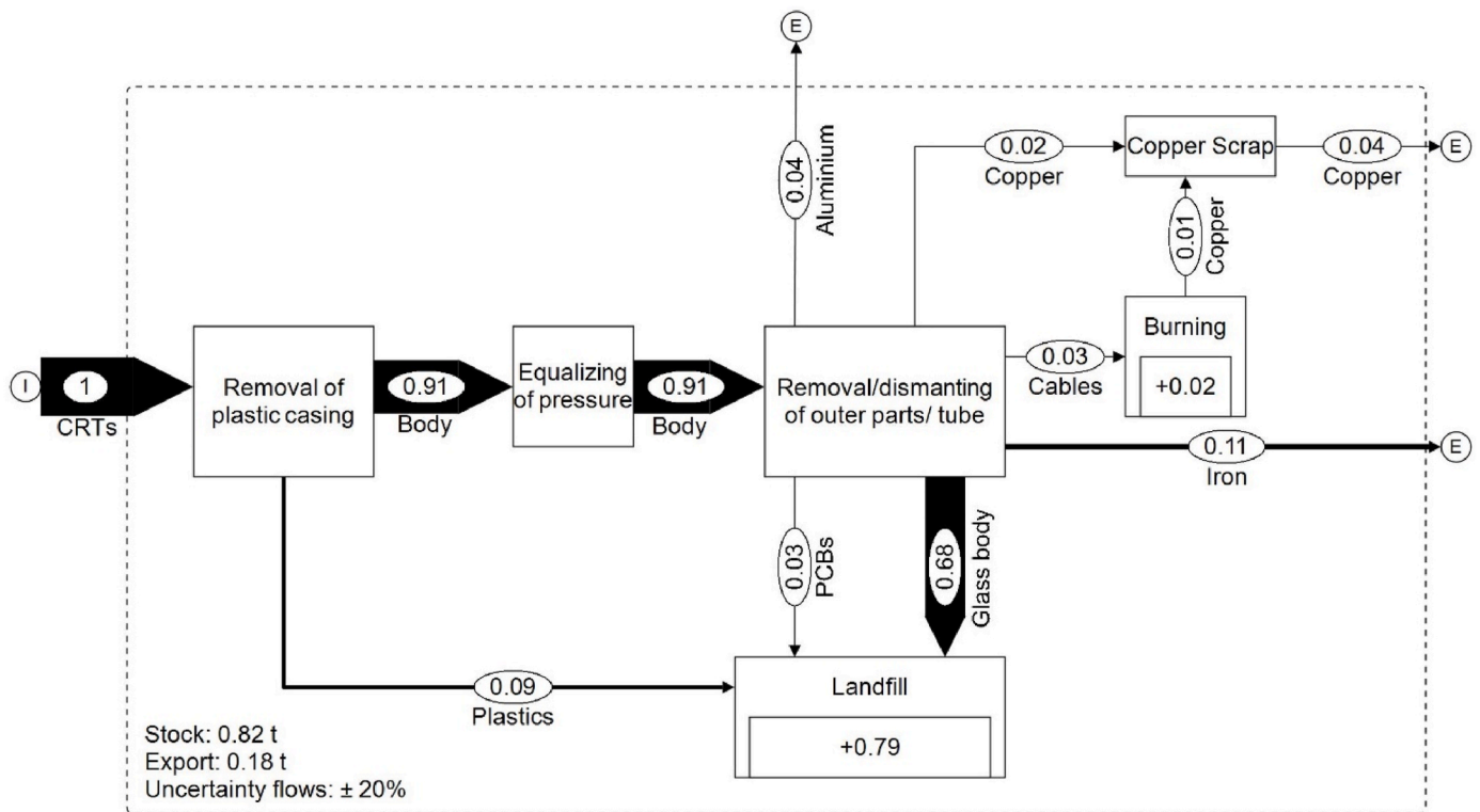
Fig. 6. Process flow of CRT dismantling in the informal sector.
