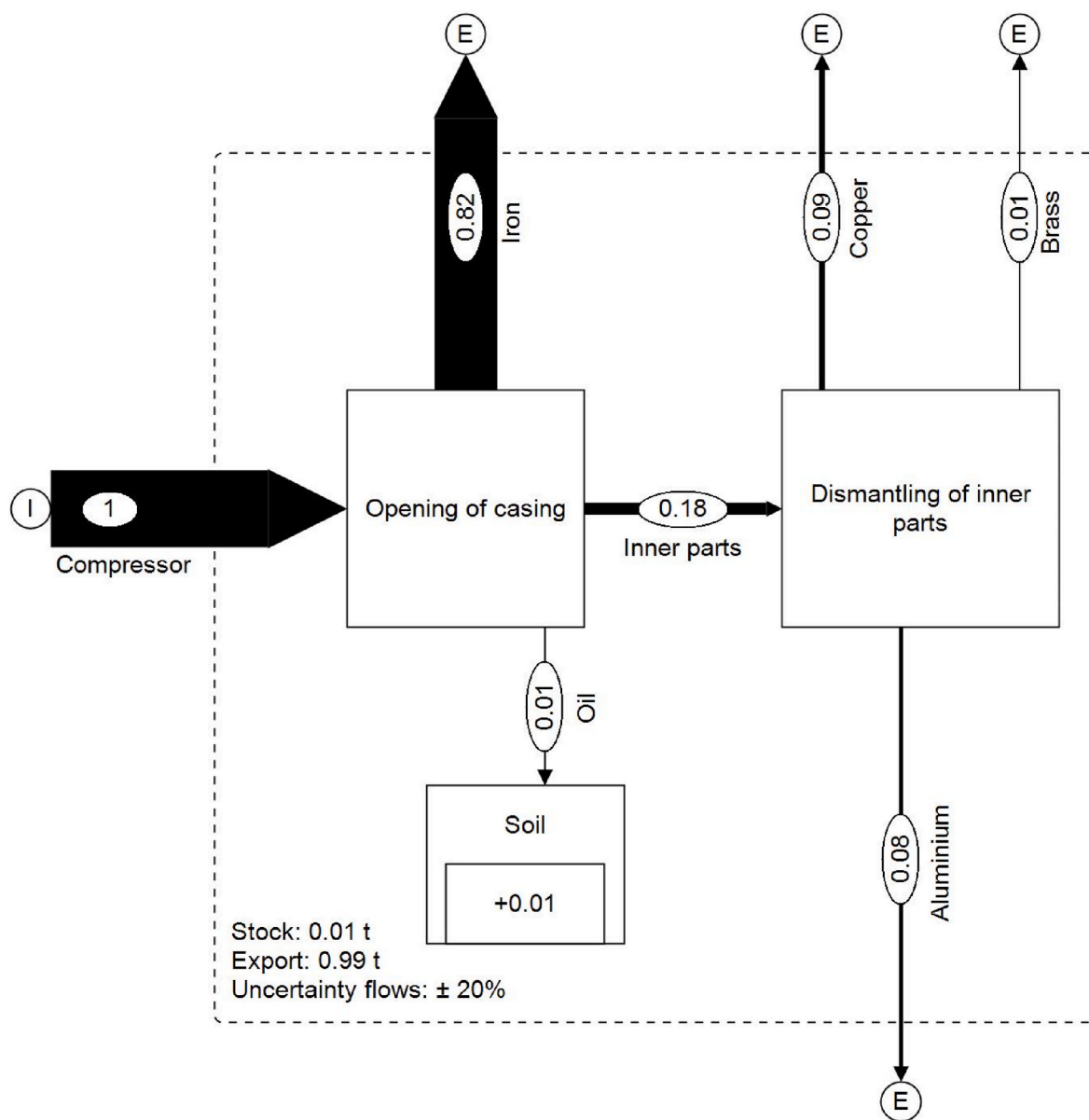
Fig. 7. Process flow of compressor dismantling in the informal sector.
