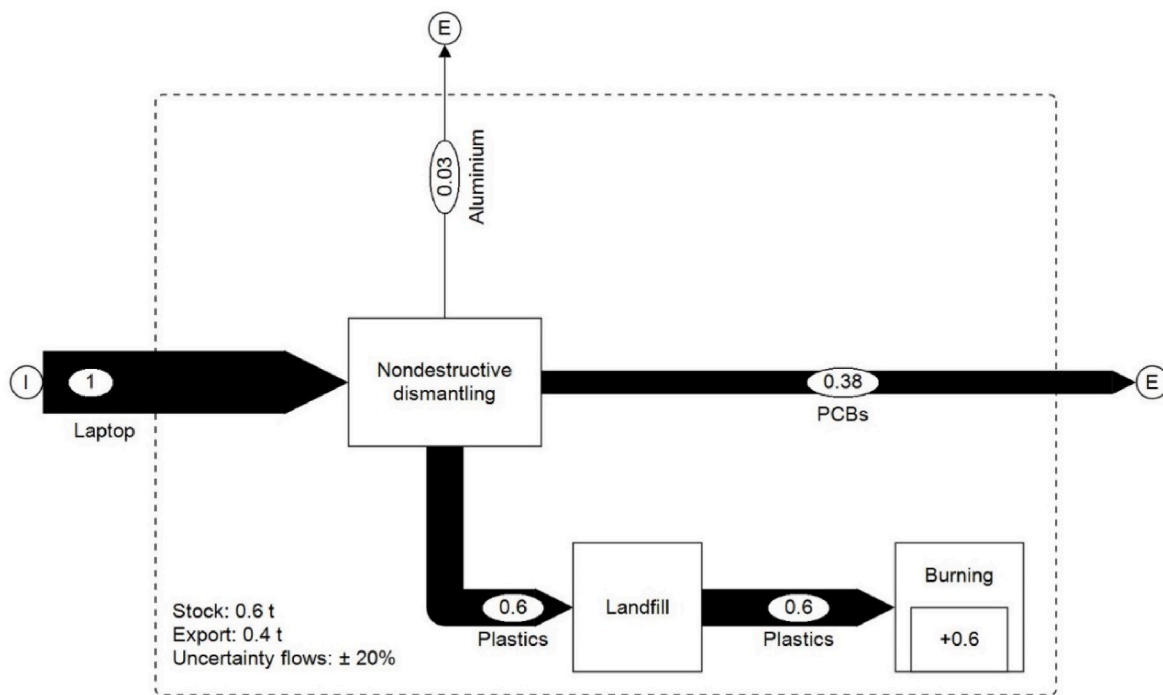
Fig. 4. Process flow of laptop dismantling in the informal sector.
