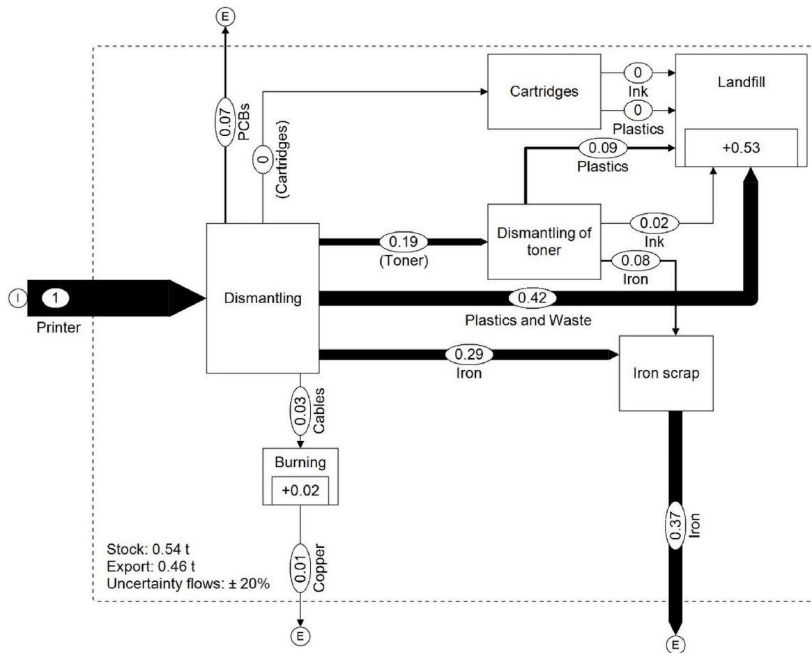
Fig. 9. Process flow of printer dismantling in the informal sector.
