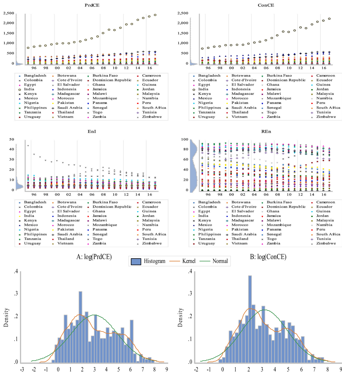
Figure-1. a. Distributional Plots of Key Variables. b. Distributional -Kernel and Normality Plots of CO 2 Emissions.
