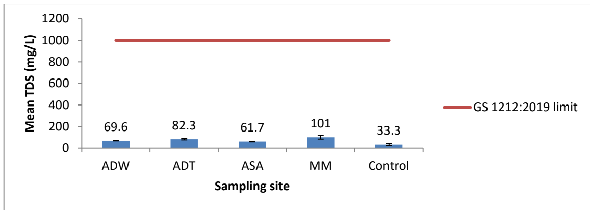
Figure 6: TDS Variations across surface water locations, Mpohor Wassa East District
