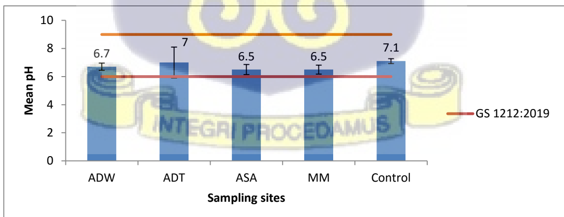
Figure 4: pH Variations across surface water locations, Mpohor Wassa East
