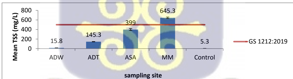
Figure 7: TSS Variations across surface water locations, Mpohor Wassa East District
