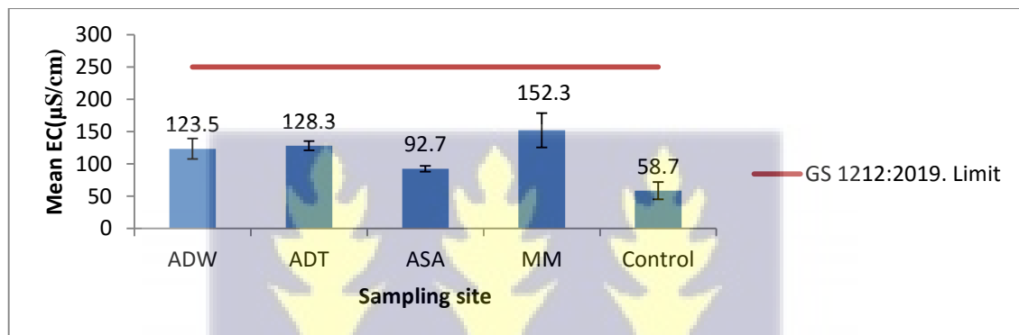
Figure 5: Conductivity Variations across surface water locations, Mpohor Wassa East
