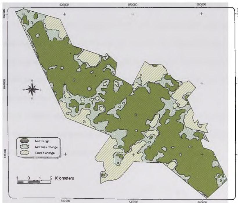
Figure 5.9 c Image Differencing Change map of Tinte Bepo Forest Reserve.
