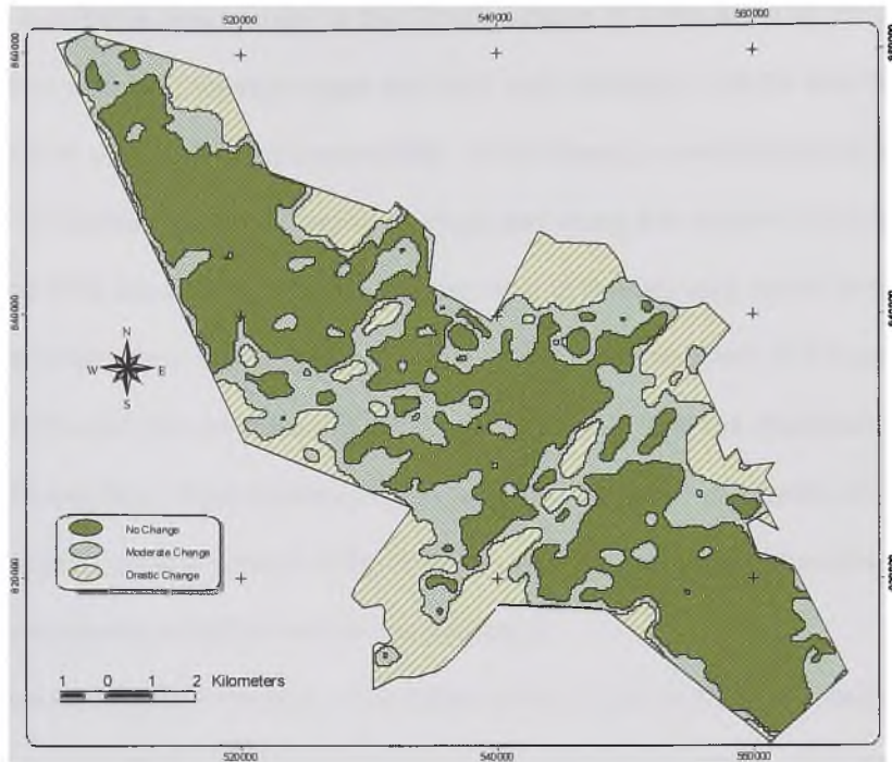
Figure 5.9 b Spectral Temporal PCA Change map of Tinte Bepo Forest Reserve.
