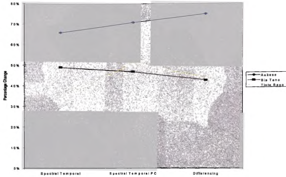
Figure 5.6 Identification of Trends in Change Detection Methods.
