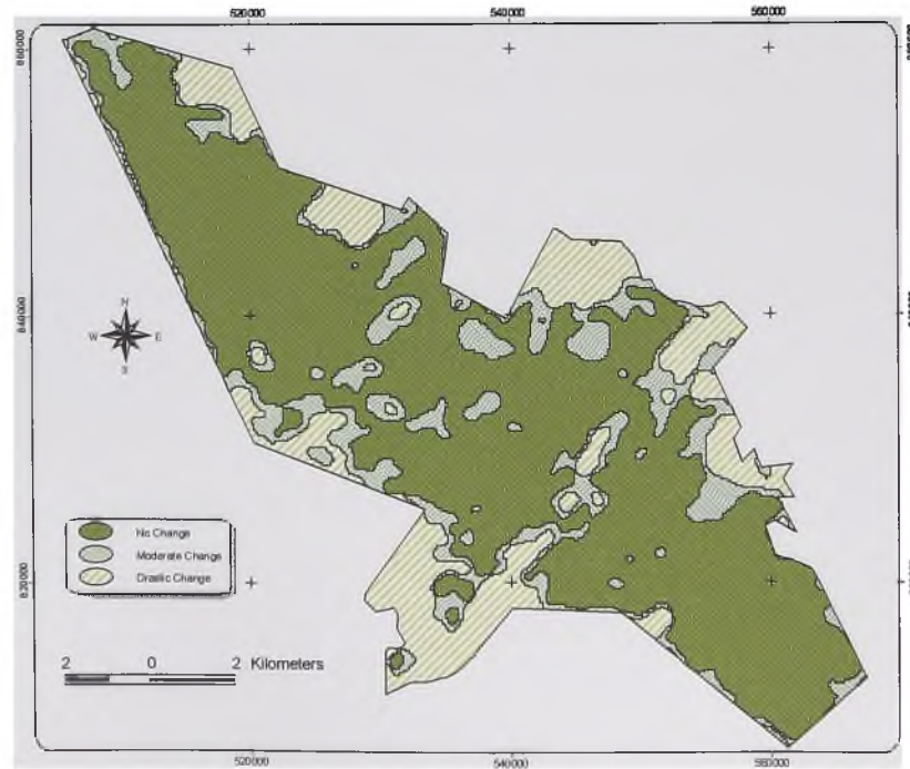
Figure 5.9 a Spectral Temporal Change map of Tinte Bepo Forest Reserve
