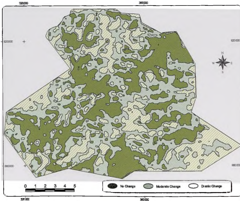
Figure 5.7 a Spectral Temporal Change map of Asukese.
