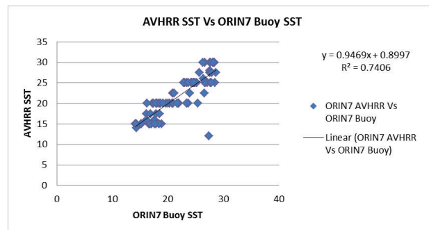
Figure 7: Linear regression analysis of AVHRR SST Vs. ORIN7 Buoy SST
