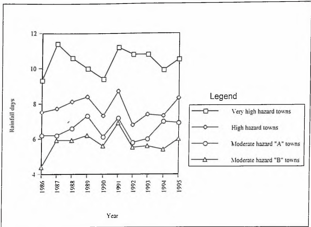
Figure 3. Mean annual rainfall days >0.25 mm over a 10-year period for the four hazard zones.
