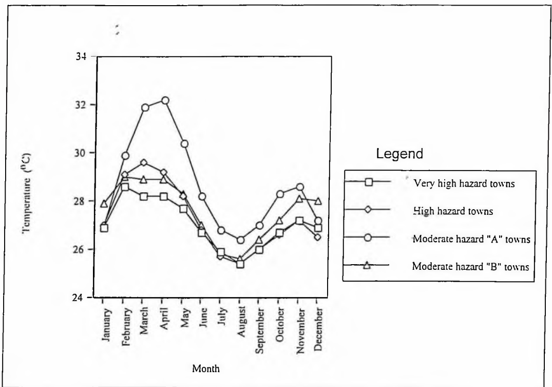
Figure 6. Annual temperature trend for the four decay hazard zones.
