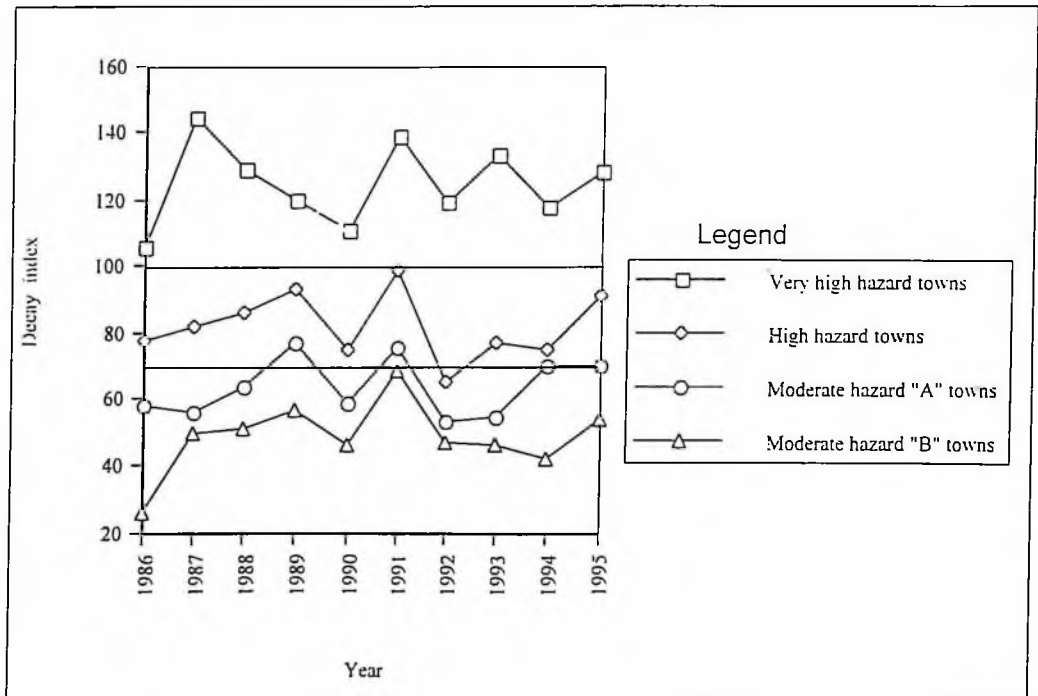
Figure 2. Annual decay index variation for the four decay hazard zones.
