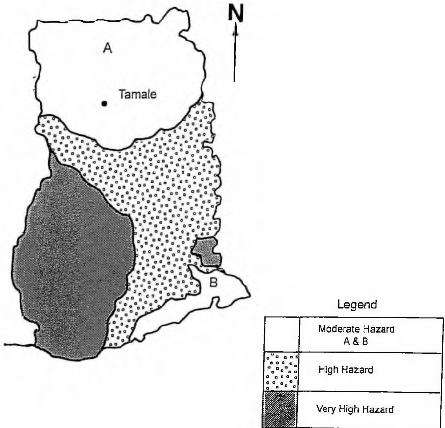
Figure 7. Wood decay hazard potential for Ghana.
