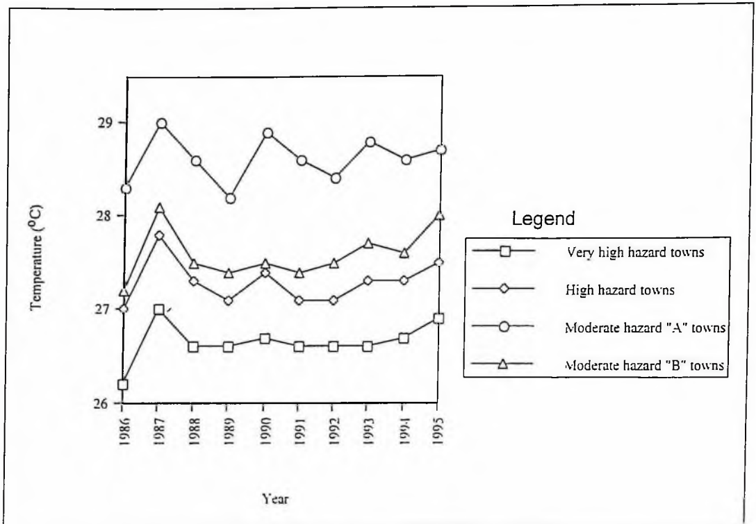
Figure 4. Mean annual temperature for the four hazard zones over a 10-year period.
