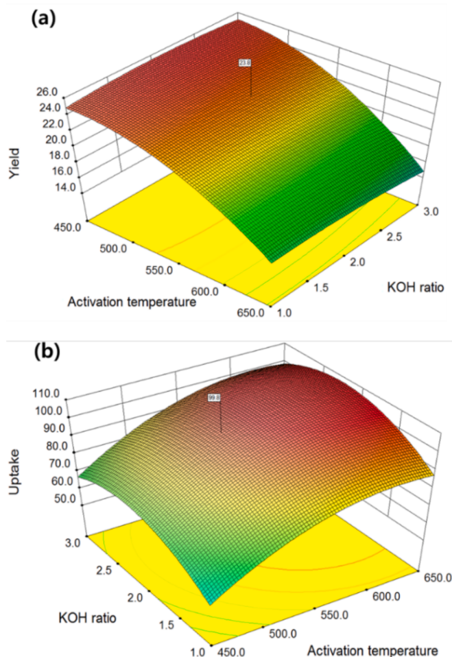
Fig. 3. Three-dimensional (3D) surface plots of numerically optimized factors and desired responses; (a) yield and (b) uptake responses.
