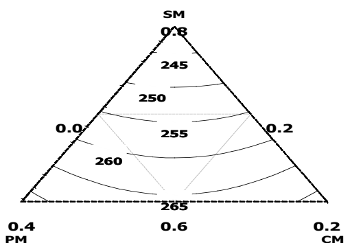
Figure 6. contour plot of energy value of SPCM formulations
