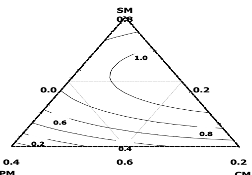
Figure 7. contour plot of carbohydrate content of SPCM formulations
