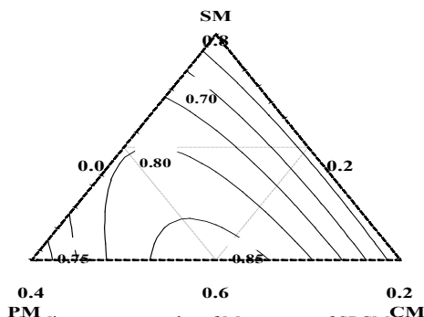
Figure 11: Mixture contour plot of Mn content of SPCM formulations
