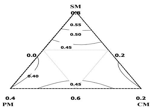
Figure 8. contour plot of ash content of SPCM formulations
