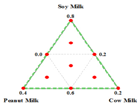
Figure 1. constrained simplex design used in formulating ingredients for vegetable milk yoghurt
