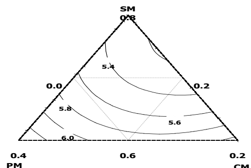
Figure 5. contour plot of fat content of SPCM formulations
