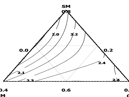
Figure 4. contour plot of protein content of SPCM formulations
