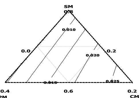
Figure 14. contour plot of titratable acidity of SPCM formulations
