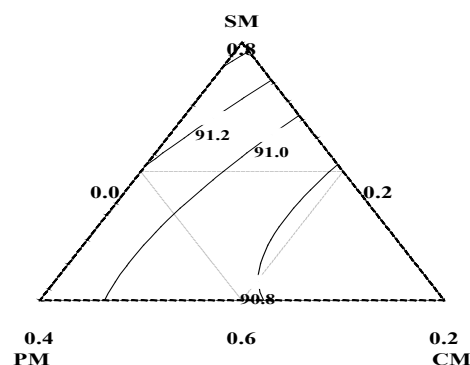
Figure 3. contour plot of moisture content of SPCM formulations
