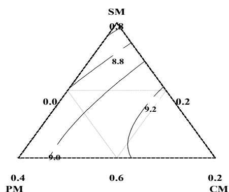
Figure 2. contour plot of total solids content of SPCM formulations
