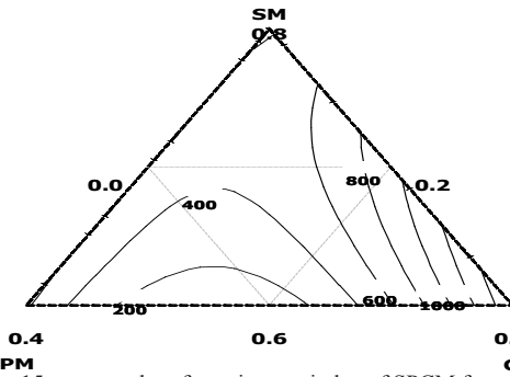
Figure 15. contour plot of consistency index of SPCM formulations
