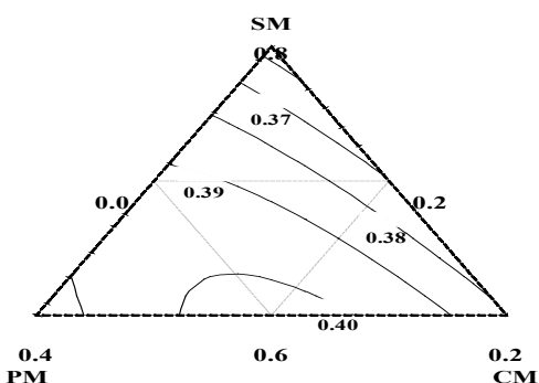
Figure 10: Mixture contour plot of Zn content of SPCM formulations
