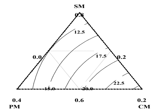
Figure 9. Mixture contour plot of Ca content of SPCM formulations
