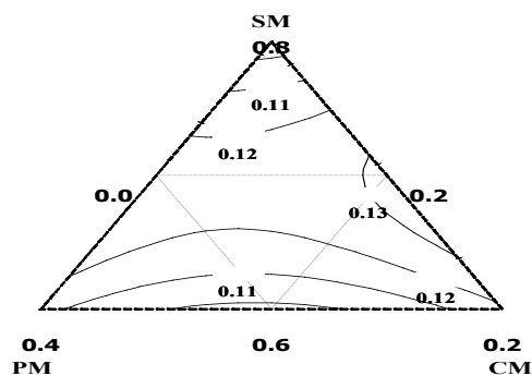
Figure 12. contour plot of Fe content of SPCM formulations
