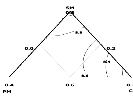
Figure 13. contour plot of pH of SPCM formulations
