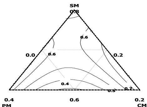
Figure 16. contour plot of flow behaviour indices of SPCM formulations
