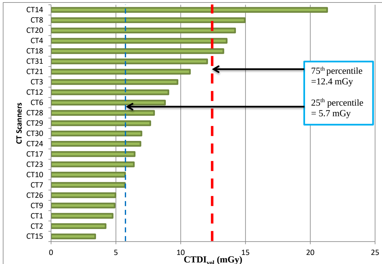
Figure 4. 12: Distribution of representative CTDI vol values for lung tumour/cancer CT indication
