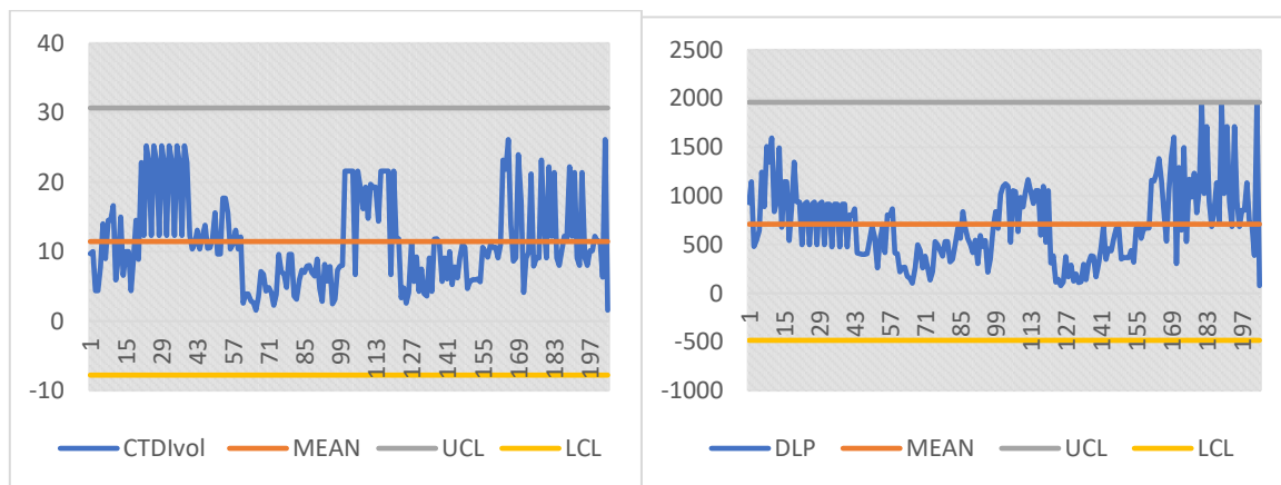
Figure 9: Control chart for PE data sets (CTDI vol and DLP)
