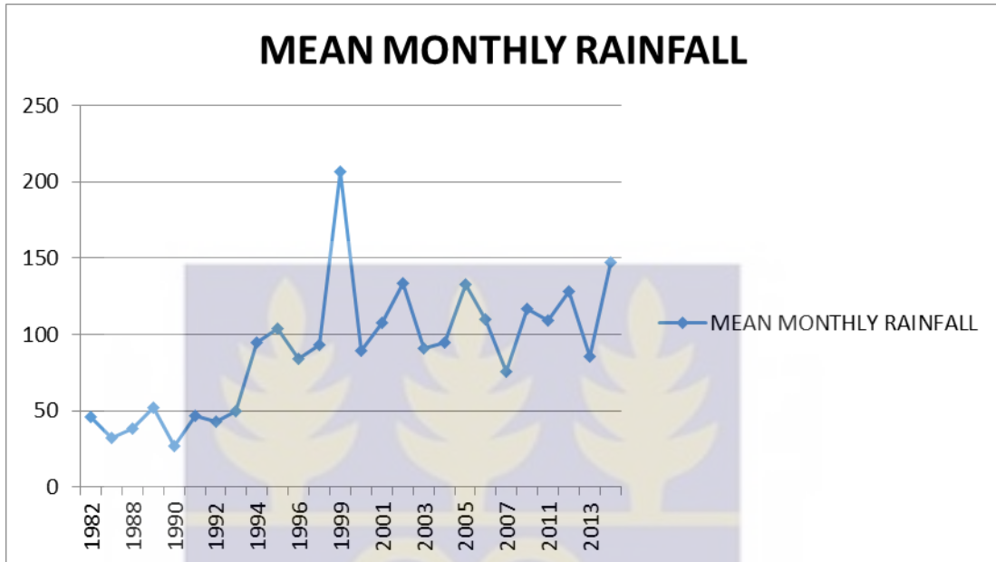
Figure 3.2 Mean monthly rainfall the Lawra District from the Ghana (Source: Ghana Meteorological Agency)
