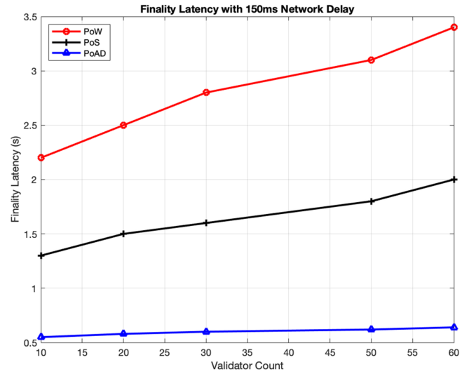
FIGURE 14 | Finality latency (in seconds) under network delay (150 ms) across different consensus protocols.
