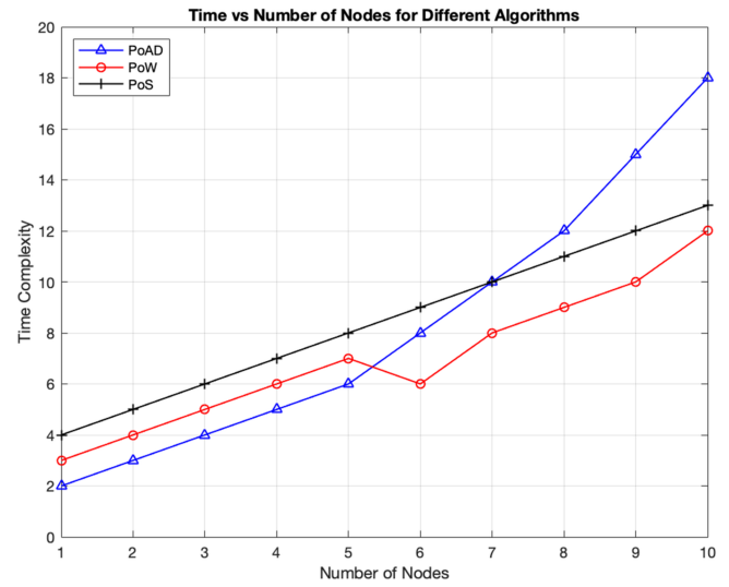
FIGURE 6 | Time complexity across PoW, PoS, and PoAD.
