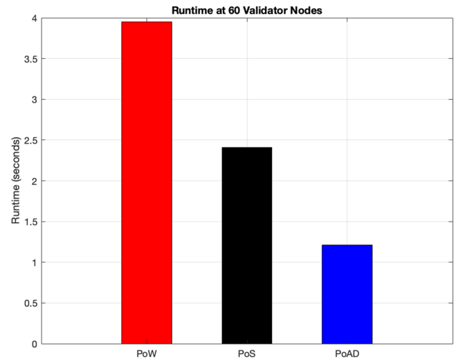
FIGURE 9 | Runtime performance of PoW, PoS, and PoAD at 60 validator nodes.
