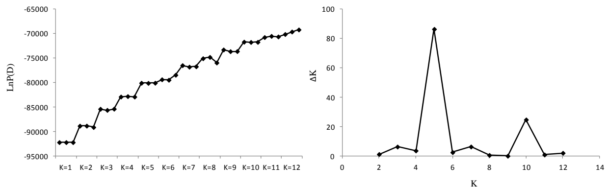
Figure 4. 2. Analysis of the population structure of 96 maize inbred lines. Changing trends of estimated L_n probability of data ( L_n P(D) ) and Pritchard's K ( \Delta K ) over three repeats at each K value in the STRUCTURE analysis are shown.
