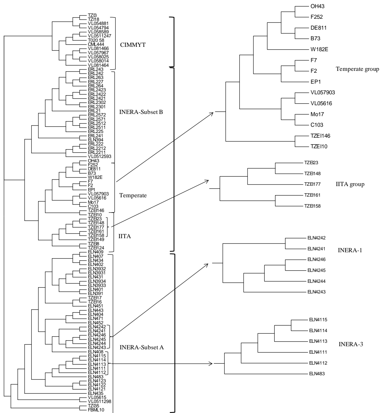
Figure 4. 5. Neighbor-joining (NJ) tree for the 96 maize inbred lines based on Roger’s genetic distance. A sectional tree representing Temperate, IITA, INERA-1 and INERA-3 groups identified in the structure analysis are shown in the right. Inbreds codes are presented in Table S1 (Appendices).
