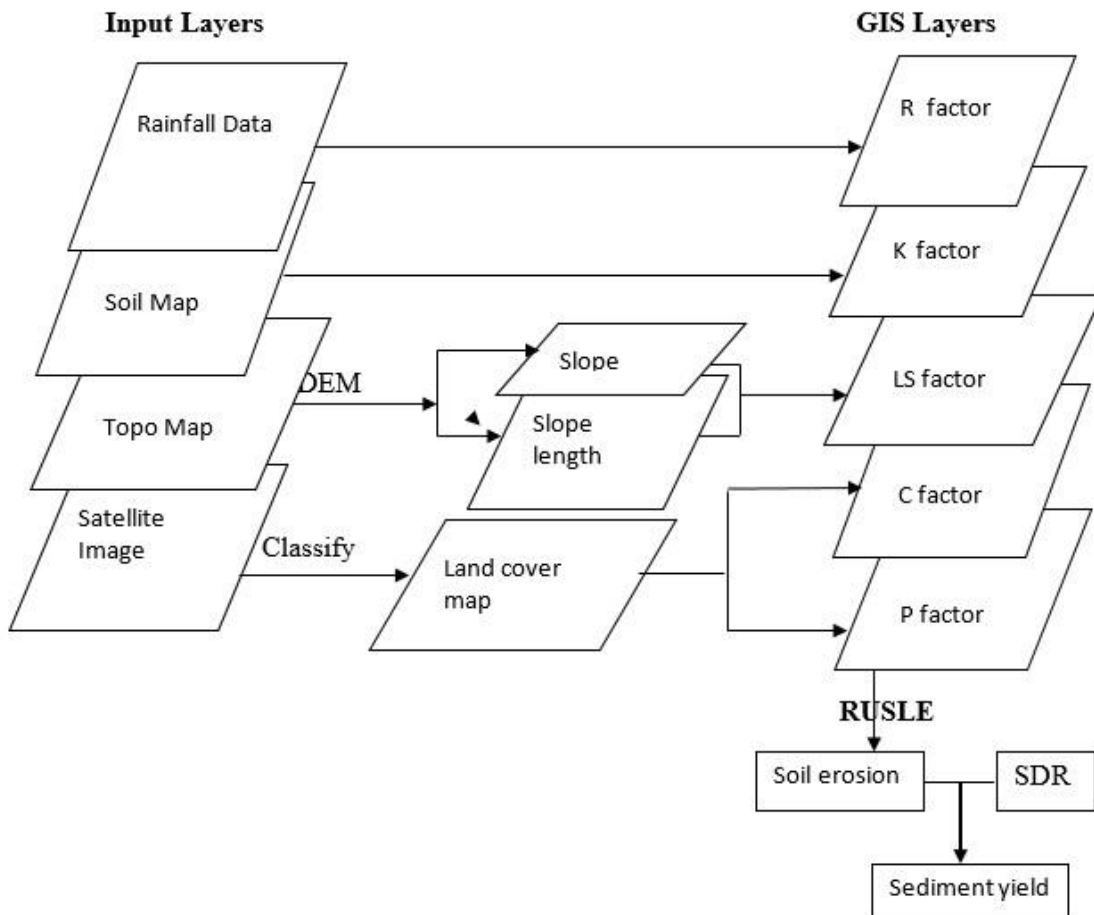
Fig.2: Schematic chart of GIS applications to soil erosion mapping and the derivation of Sediment Delivery Ratio - SDR (Modified from Mongkolsawat et al. 1994).
