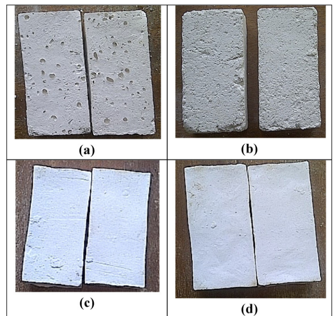
Fig. 10. Sintered bodies at 1150\text{ }^\circ\text{C} . a) Sample with styrofoam b) Sample with PHDPE c) Sample with sawdust d) Sample without pore formers.
