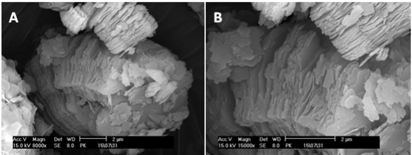
Plate II. SEM images of beneficiated Kankara kaolin at magnifications of (A) 8000× (B) 15,000×.
