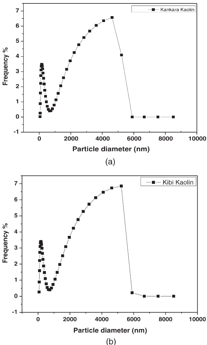
Fig. 2. Particle size distribution of Kankara and Kibi Kaolin.
