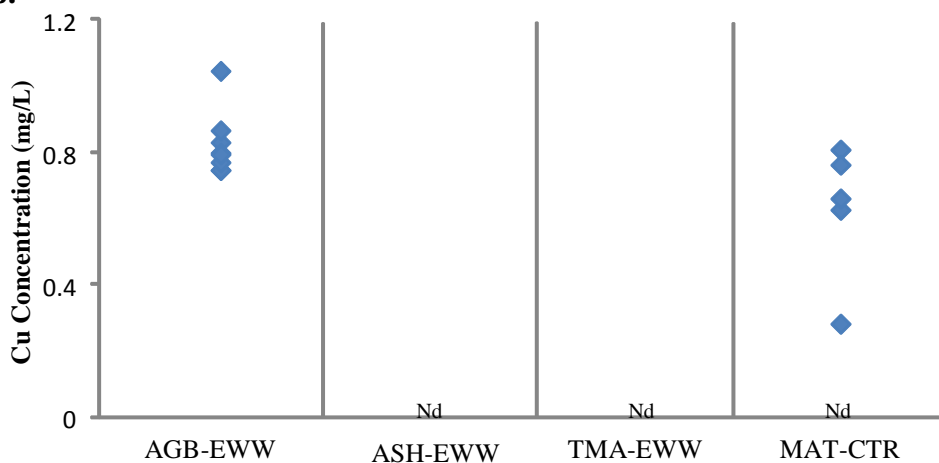
Figure 5.9: Comparison of Cu concentrations in urine of e-waste workers with control group.
