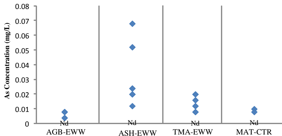
Figure 5.13: Comparison of As concentrations in urine of e-waste workers with control group.
