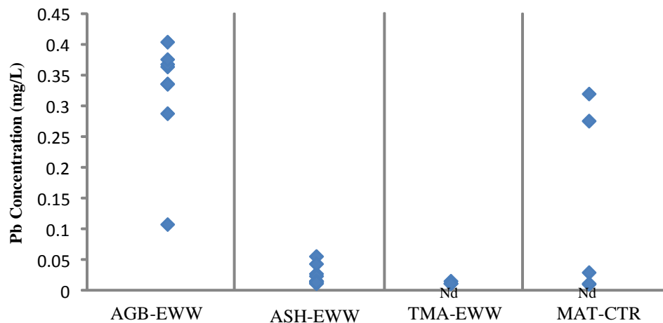
Figure 5.12: Comparison of Pb concentrations in urine of e-waste workers with control group.
