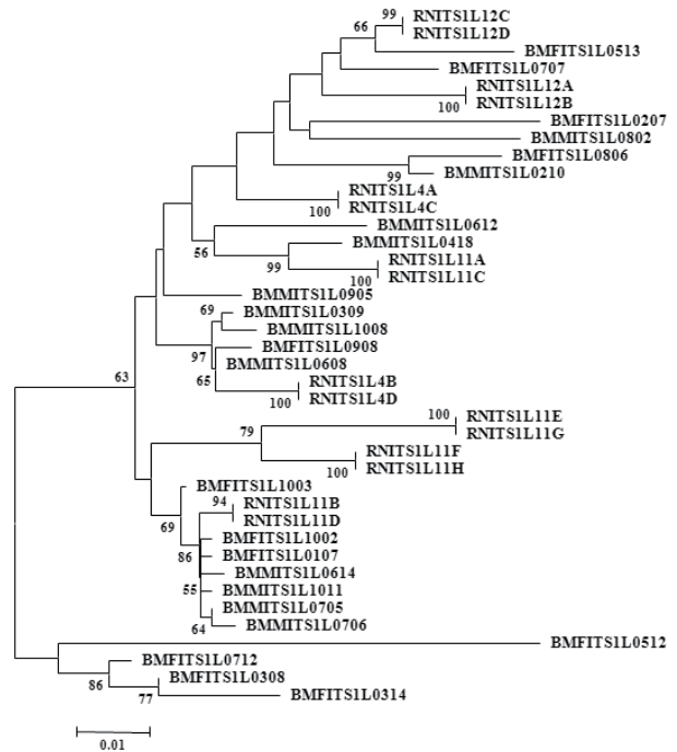
Figure 4. Phylogram generated from Neighbor-Joining analysis for ITS1-720 sequences for female and male reniform nematodes from mixed-Alabama and Belle Mina populations. The percentages of bootstrap replicates supporting the clades are indicated at the branch points. Bootstrap values greater than 50% are shown beside nodes. RN= Reniform nematode; ITS1L= Large ITS1 rDNA; 01-10 = reniform nematode isolate IDs; A, B, C, D, E, F, G, H/01-18= clone IDs, BM=Belle Mina, F=Female, M=Male.
