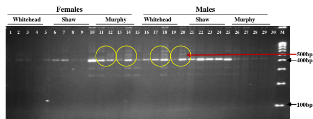
Figure 1. Restriction Fragment Length Polymorphism from the digestion of ITS1 region of 5 female and five male reniform nematodes in three locations - WhiteHead (W), Shaw (S), and Murphy (R) digested using the restriction enzyme MspI and separated on 6% Polyacrylamide Gel (PAGE). Circled regions show presence of 500 bp bands among the amplicons. Lane M=100bp marker.
